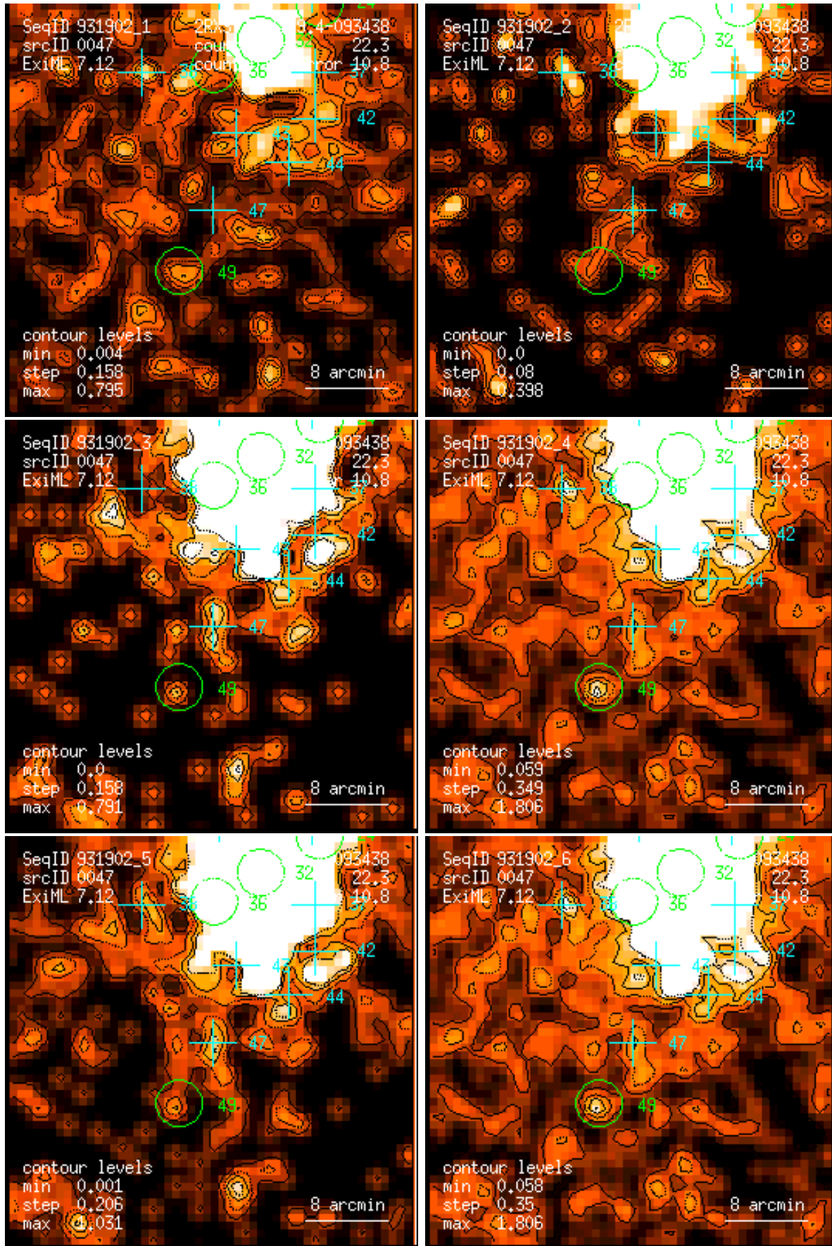
Figure 47: RASS 931902: detection 0047: band rate images, Gaussian filter: (1) PSPC channels 11 – 41, (2) 52 – 90, (3) 91 – 201, (4) 11 – 235, (5) 52 – 201, (6) 11 – 201. Broad band rates in counts/ks. Band rate contour levels in counts/ks/arcmin 2 .
