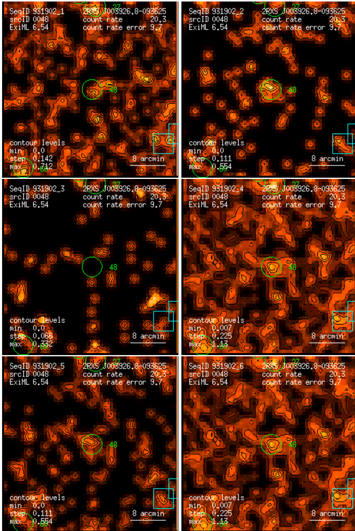
Figure 48: RASS 931902: detection 0048: band rate images, Gaussian filter: (1) PSPC channels 11 – 41, (2) 52 – 90, (3) 91 – 201, (4) 11 – 235, (5) 52 – 201, (6) 11 – 201. Broad band rates in counts/ks. Band rate contour levels in counts/ks/arcmin 2 .
