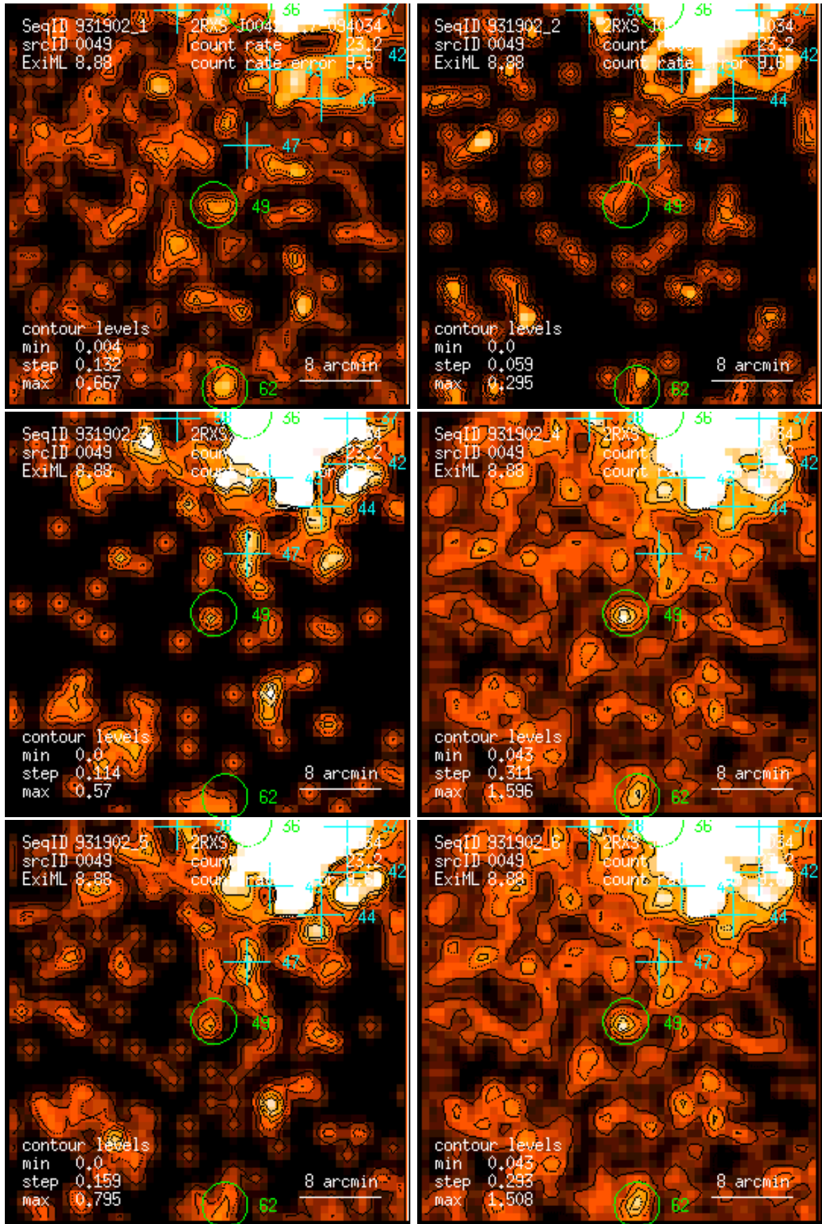
Figure 49: RASS 931902: detection 0049: band rate images, Gaussian filter: (1) PSPC channels 11 – 41, (2) 52 – 90, (3) 91 – 201, (4) 11 – 235, (5) 52 – 201, (6) 11 – 201. Broad band rates in counts/ks. Band rate contour levels in counts/ks/arcmin 2 .
