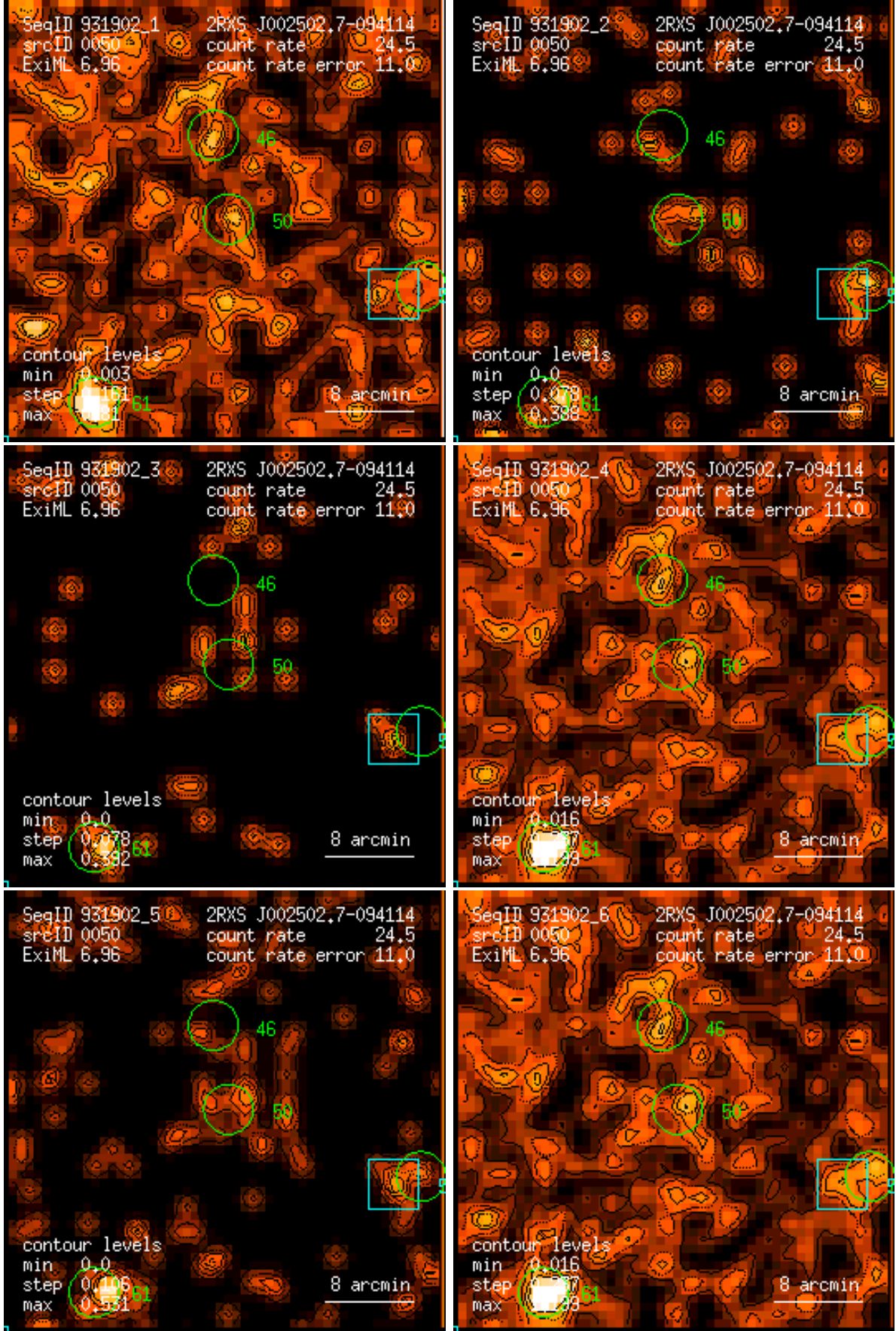
Figure 50: RASS 931902: detection 0050: band rate images, Gaussian filter: (1) PSPC channels 11 – 41, (2) 52 – 90, (3) 91 – 201, (4) 11 – 235, (5) 52 – 201, (6) 11 – 201. Broad band rates in counts/ks. Band rate contour levels in counts/ks/arcmin 2 .
