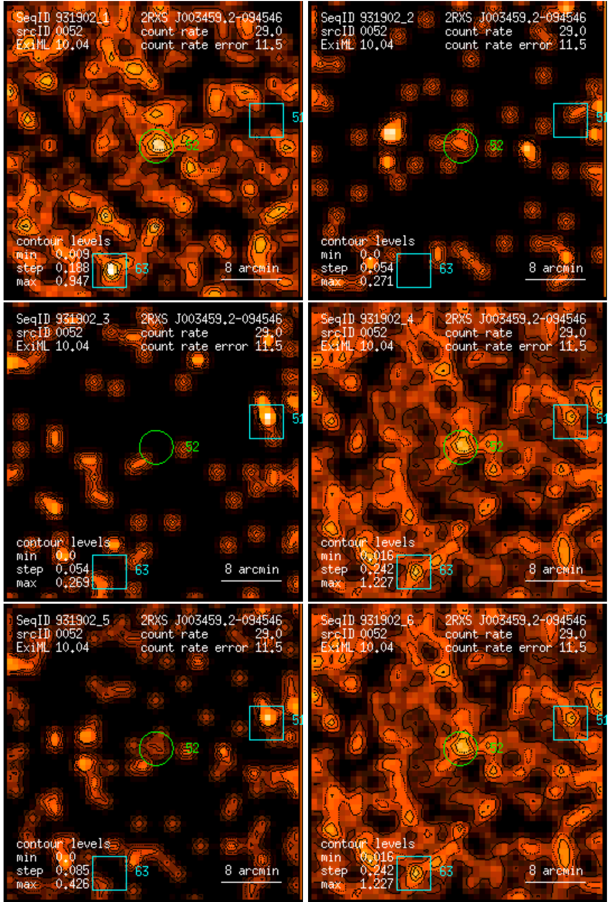
Figure 52: RASS 931902: detection 0052: band rate images, Gaussian filter: (1) PSPC channels 11 – 41, (2) 52 – 90, (3) 91 – 201, (4) 11 – 235, (5) 52 – 201, (6) 11 – 201. Broad band rates in counts/ks. Band rate contour levels in counts/ks/arcmin 2 .
