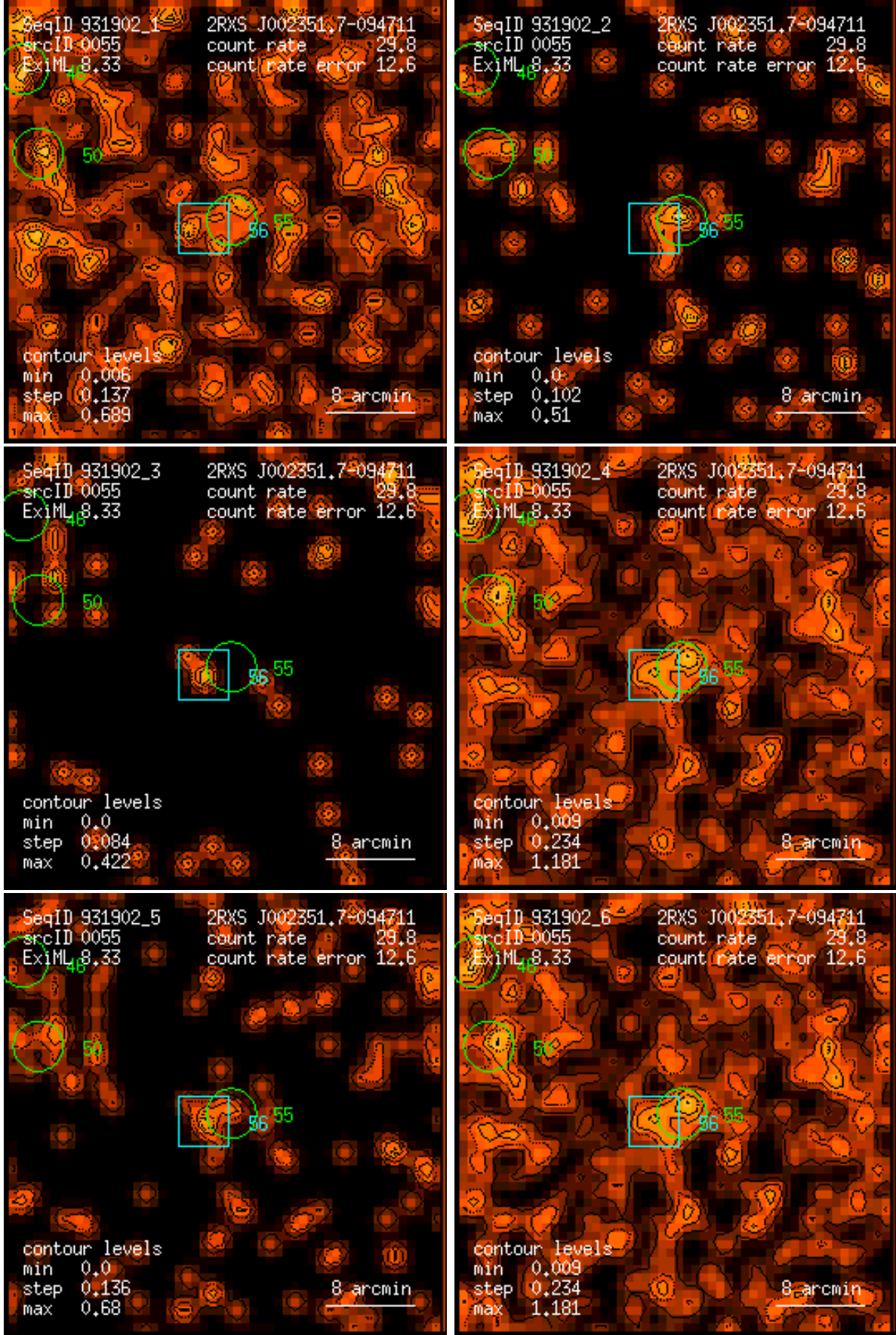
Figure 55: RASS 931902: detection 0055: band rate images, Gaussian filter: (1) PSPC channels 11 – 41, (2) 52 – 90, (3) 91 – 201, (4) 11 – 235, (5) 52 – 201, (6) 11 – 201. Broad band rates in counts/ks. Band rate contour levels in counts/ks/arcmin 2 .
