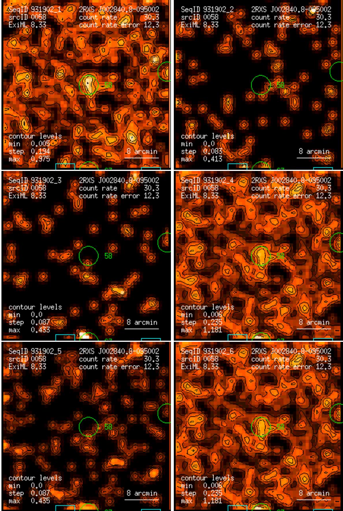
Figure 58: RASS 931902: detection 0058: band rate images, Gaussian filter: (1) PSPC channels 11 – 41, (2) 52 – 90, (3) 91 – 201, (4) 11 – 235, (5) 52 – 201, (6) 11 – 201. Broad band rates in counts/ks. Band rate contour levels in counts/ks/arcmin 2 .
