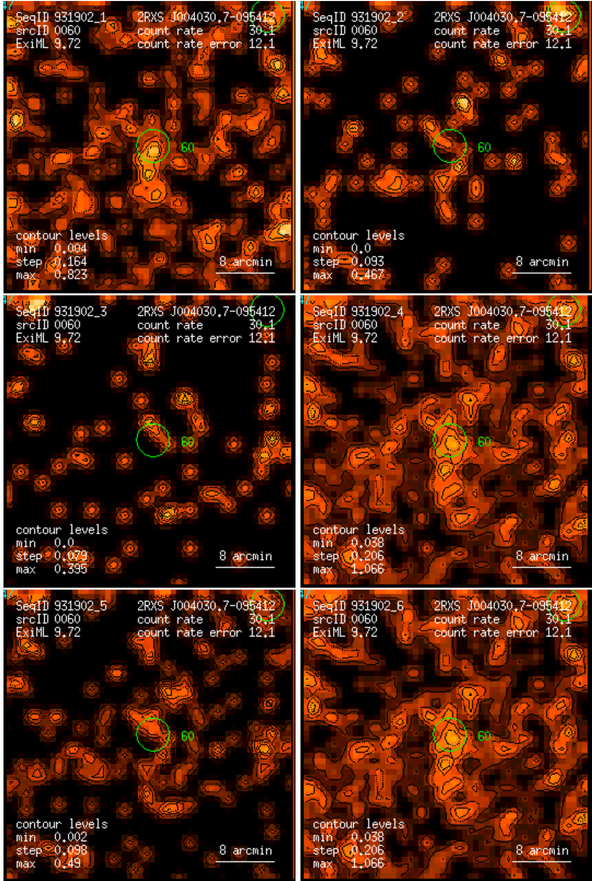
Figure 60: RASS 931902: detection 0060: band rate images, Gaussian filter: (1) PSPC channels 11 – 41, (2) 52 – 90, (3) 91 – 201, (4) 11 – 235, (5) 52 – 201, (6) 11 – 201. Broad band rates in counts/ks. Band rate contour levels in counts/ks/arcmin 2 .
