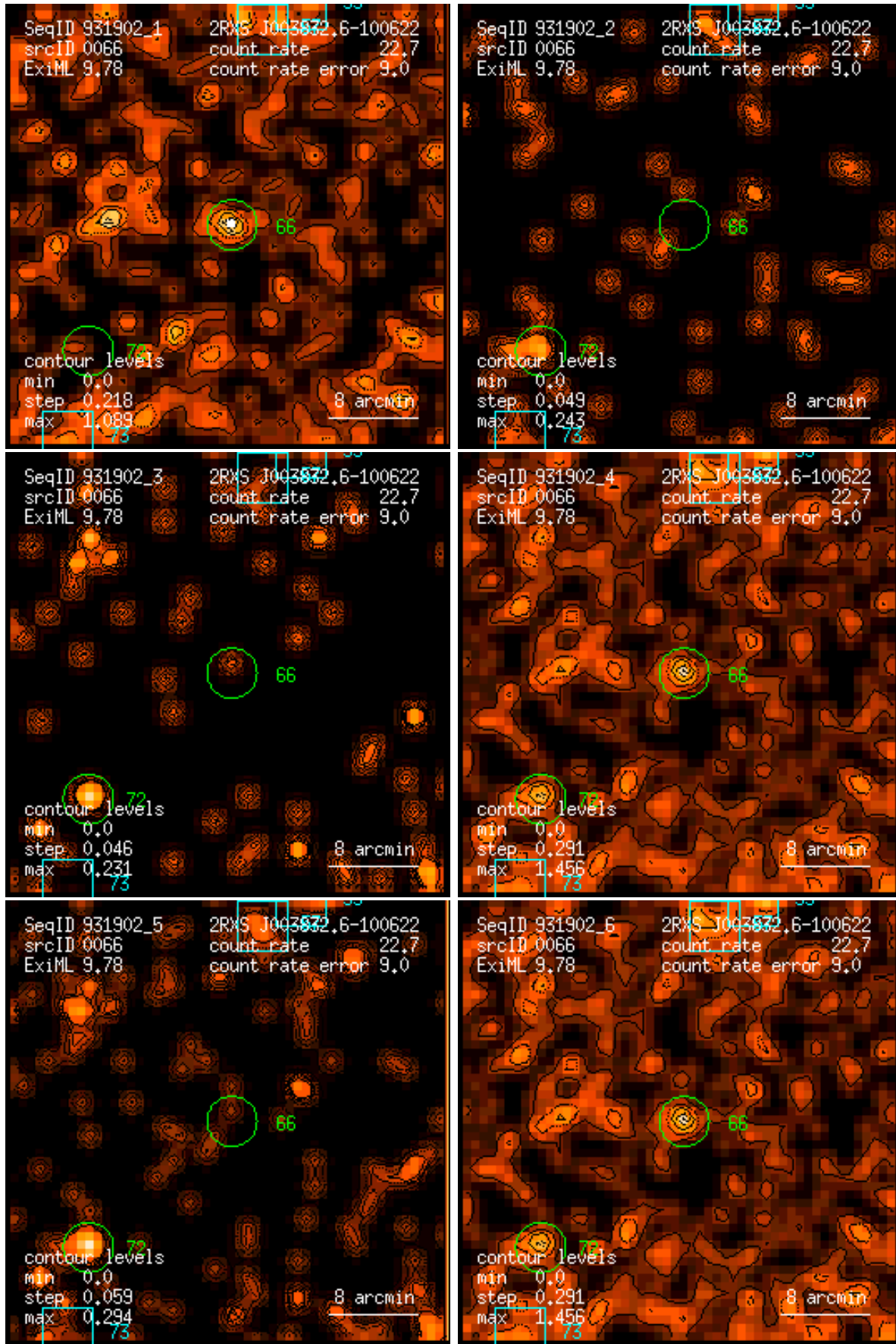
Figure 66: RASS 931902: detection 0066: band rate images, Gaussian filter: (1) PSPC channels 11 – 41, (2) 52 – 90, (3) 91 – 201, (4) 11 – 235, (5) 52 – 201, (6) 11 – 201. Broad band rates in counts/ks. Band rate contour levels in counts/ks/arcmin 2 .
