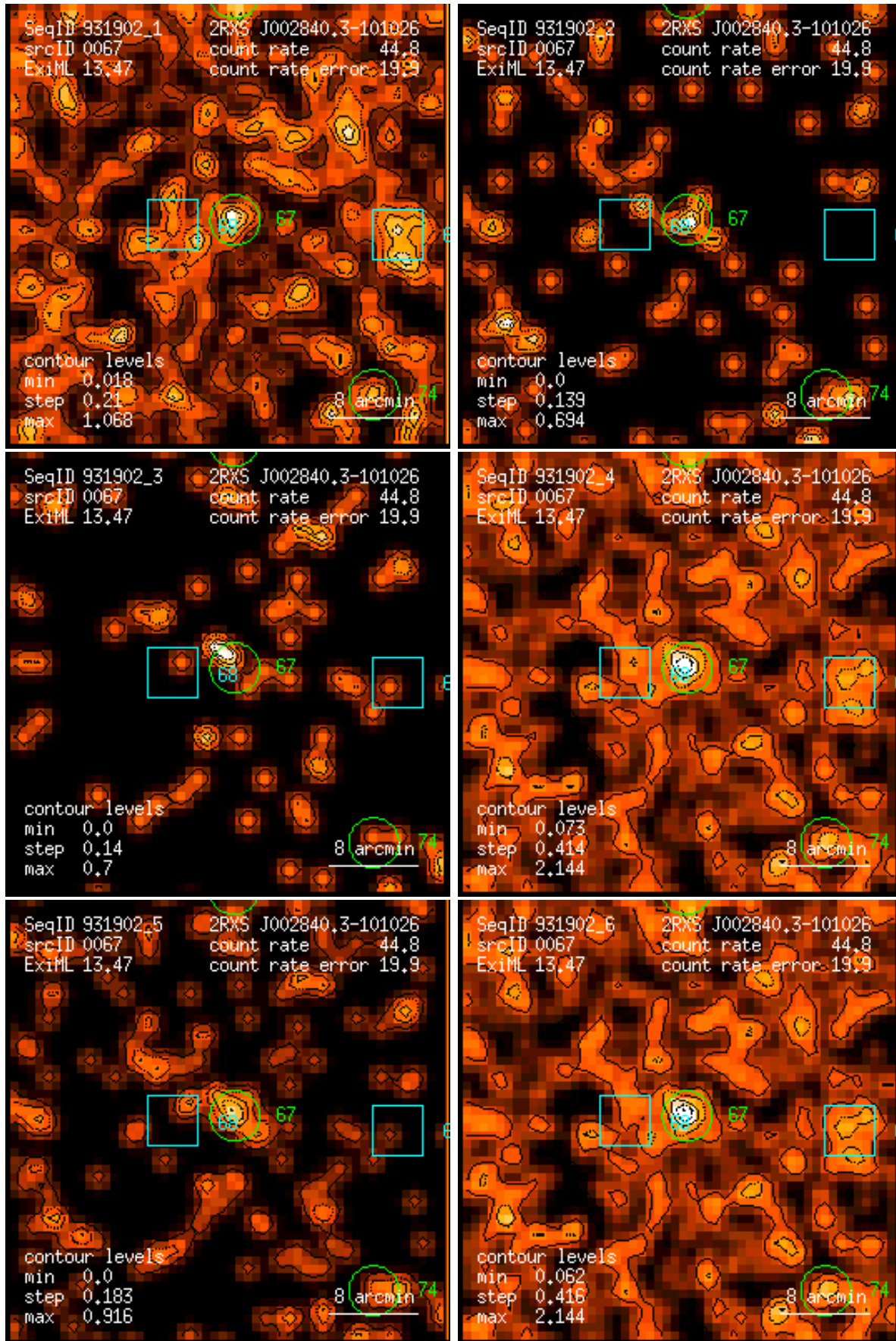
Figure 67: RASS 931902: detection 0067: band rate images, Gaussian filter: (1) PSPC channels 11 – 41, (2) 52 – 90, (3) 91 – 201, (4) 11 – 235, (5) 52 – 201, (6) 11 – 201. Broad band rates in counts/ks. Band rate contour levels in counts/ks/arcmin 2 .
