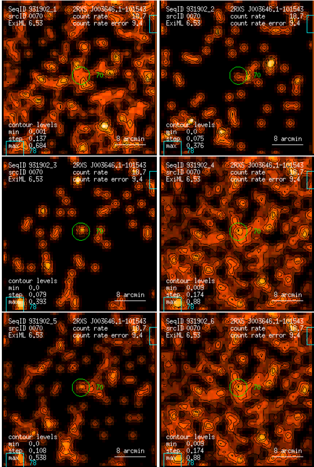
Figure 70: RASS 931902: detection 0070: band rate images, Gaussian filter: (1) PSPC channels 11 – 41, (2) 52 – 90, (3) 91 – 201, (4) 11 – 235, (5) 52 – 201, (6) 11 – 201. Broad band rates in counts/ks. Band rate contour levels in counts/ks/arcmin 2 .
