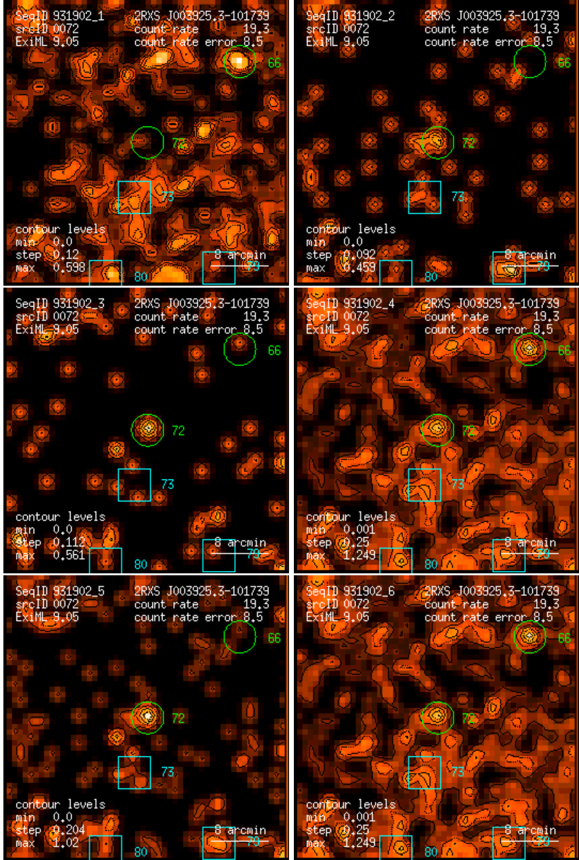
Figure 72: RASS 931902: detection 0072: band rate images, Gaussian filter: (1) PSPC channels 11 – 41, (2) 52 – 90, (3) 91 – 201, (4) 11 – 235, (5) 52 – 201, (6) 11 – 201. Broad band rates in counts/ks. Band rate contour levels in counts/ks/arcmin 2 .
