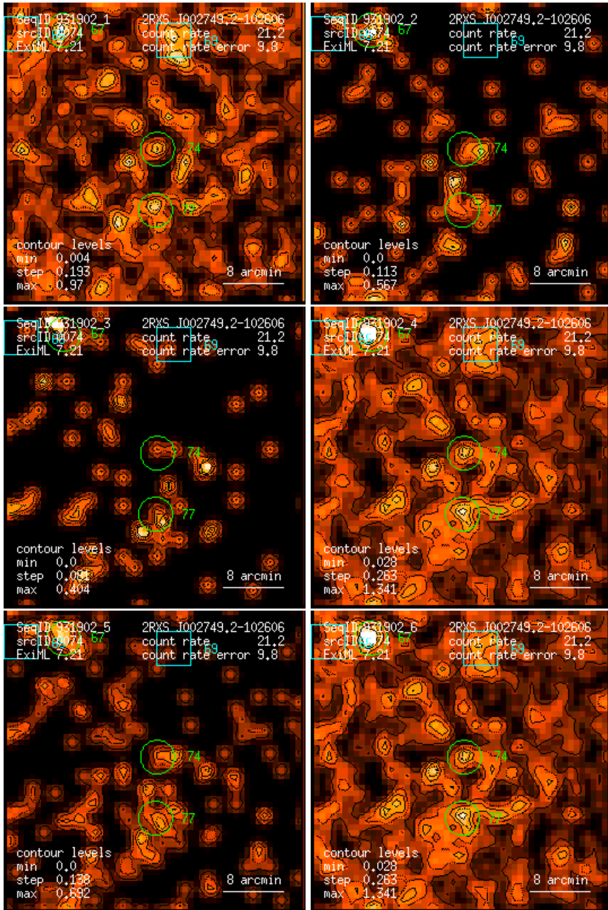
Figure 74: RASS 931902: detection 0074: band rate images, Gaussian filter: (1) PSPC channels 11 – 41, (2) 52 – 90, (3) 91 – 201, (4) 11 – 235, (5) 52 – 201, (6) 11 – 201. Broad band rates in counts/ks. Band rate contour levels in counts/ks/arcmin 2 .
