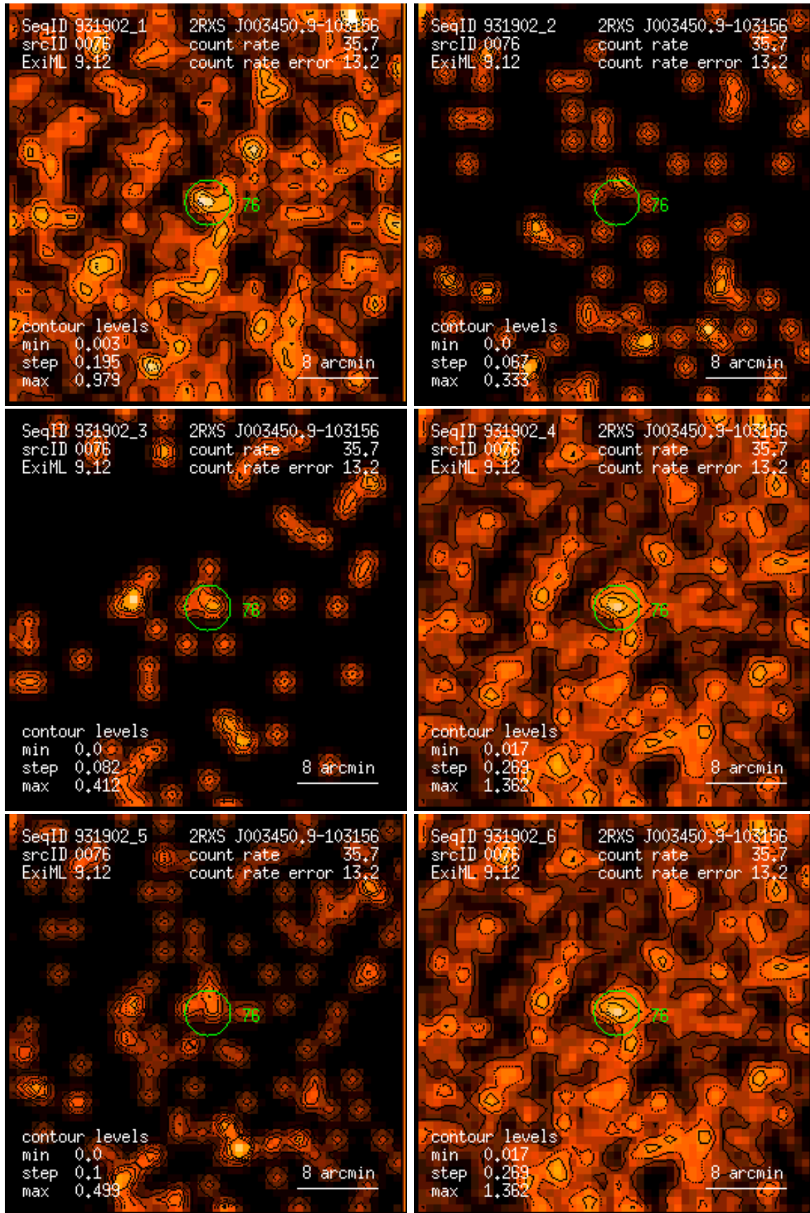
Figure 76: RASS 931902: detection 0076: band rate images, Gaussian filter: (1) PSPC channels 11 – 41, (2) 52 – 90, (3) 91 – 201, (4) 11 – 235, (5) 52 – 201, (6) 11 – 201. Broad band rates in counts/ks. Band rate contour levels in counts/ks/arcmin 2 .
