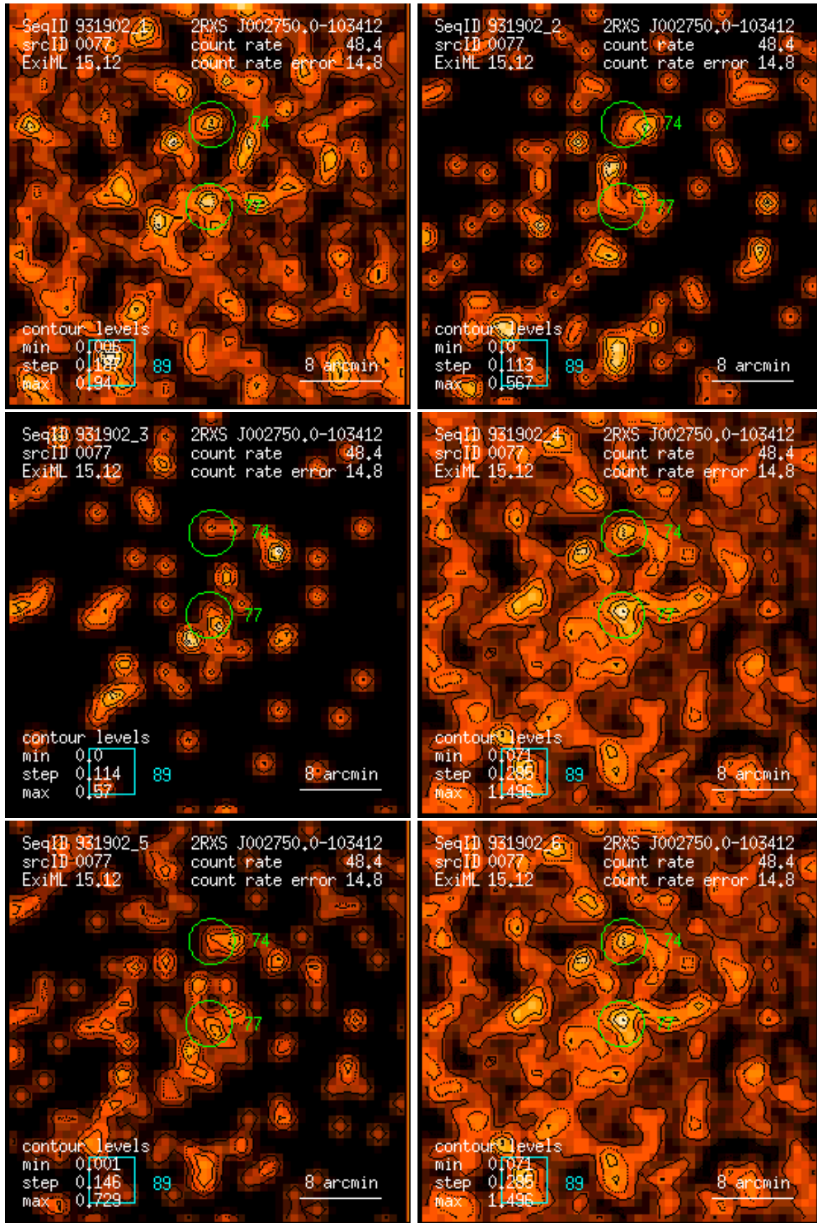
Figure 77: RASS 931902: detection 0077: band rate images, Gaussian filter: (1) PSPC channels 11 – 41, (2) 52 – 90, (3) 91 – 201, (4) 11 – 235, (5) 52 – 201, (6) 11 – 201. Broad band rates in counts/ks. Band rate contour levels in counts/ks/arcmin 2 .
