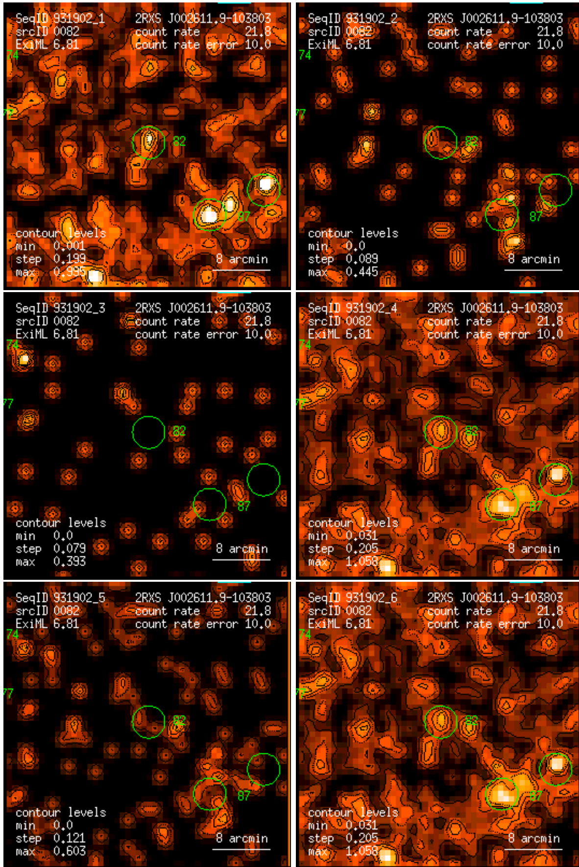
Figure 82: RASS 931902: detection 0082: band rate images, Gaussian filter: (1) PSPC channels 11 – 41, (2) 52 – 90, (3) 91 – 201, (4) 11 – 235, (5) 52 – 201, (6) 11 – 201. Broad band rates in counts/ks. Band rate contour levels in counts/ks/arcmin 2 .
