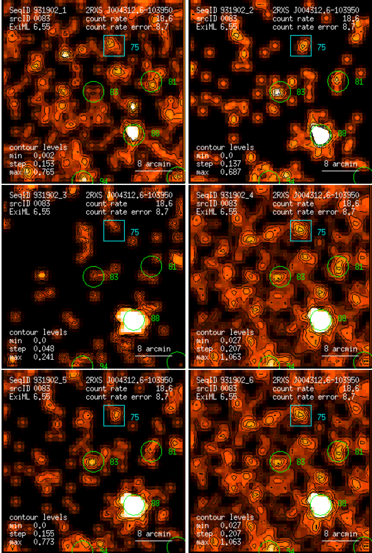
Figure 83: RASS 931902: detection 0083: band rate images, Gaussian filter: (1) PSPC channels 11 – 41, (2) 52 – 90, (3) 91 – 201, (4) 11 – 235, (5) 52 – 201, (6) 11 – 201. Broad band rates in counts/ks. Band rate contour levels in counts/ks/arcmin 2 .
