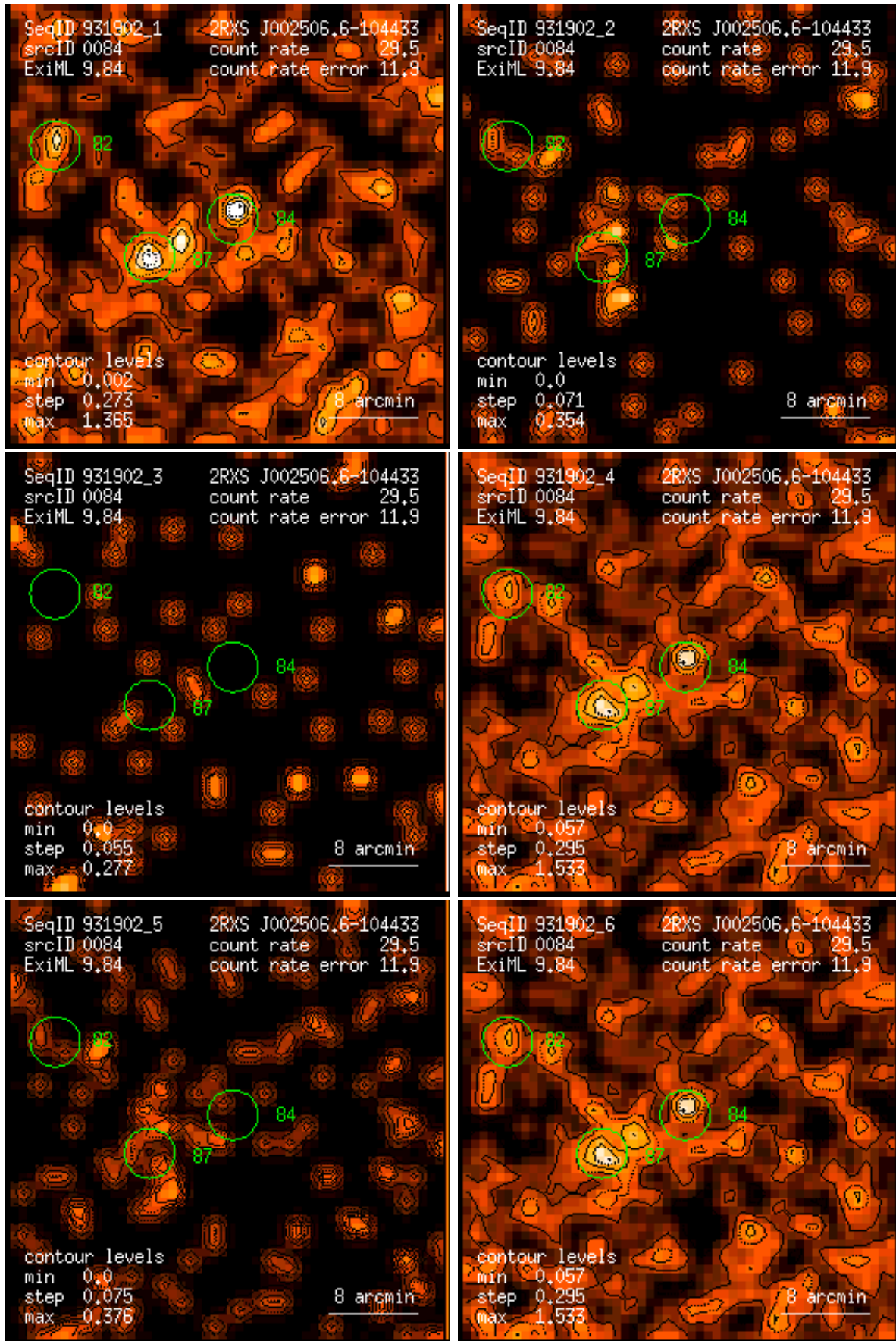
Figure 84: RASS 931902: detection 0084: band rate images, Gaussian filter: (1) PSPC channels 11 – 41, (2) 52 – 90, (3) 91 – 201, (4) 11 – 235, (5) 52 – 201, (6) 11 – 201. Broad band rates in counts/ks. Band rate contour levels in counts/ks/arcmin 2 .
