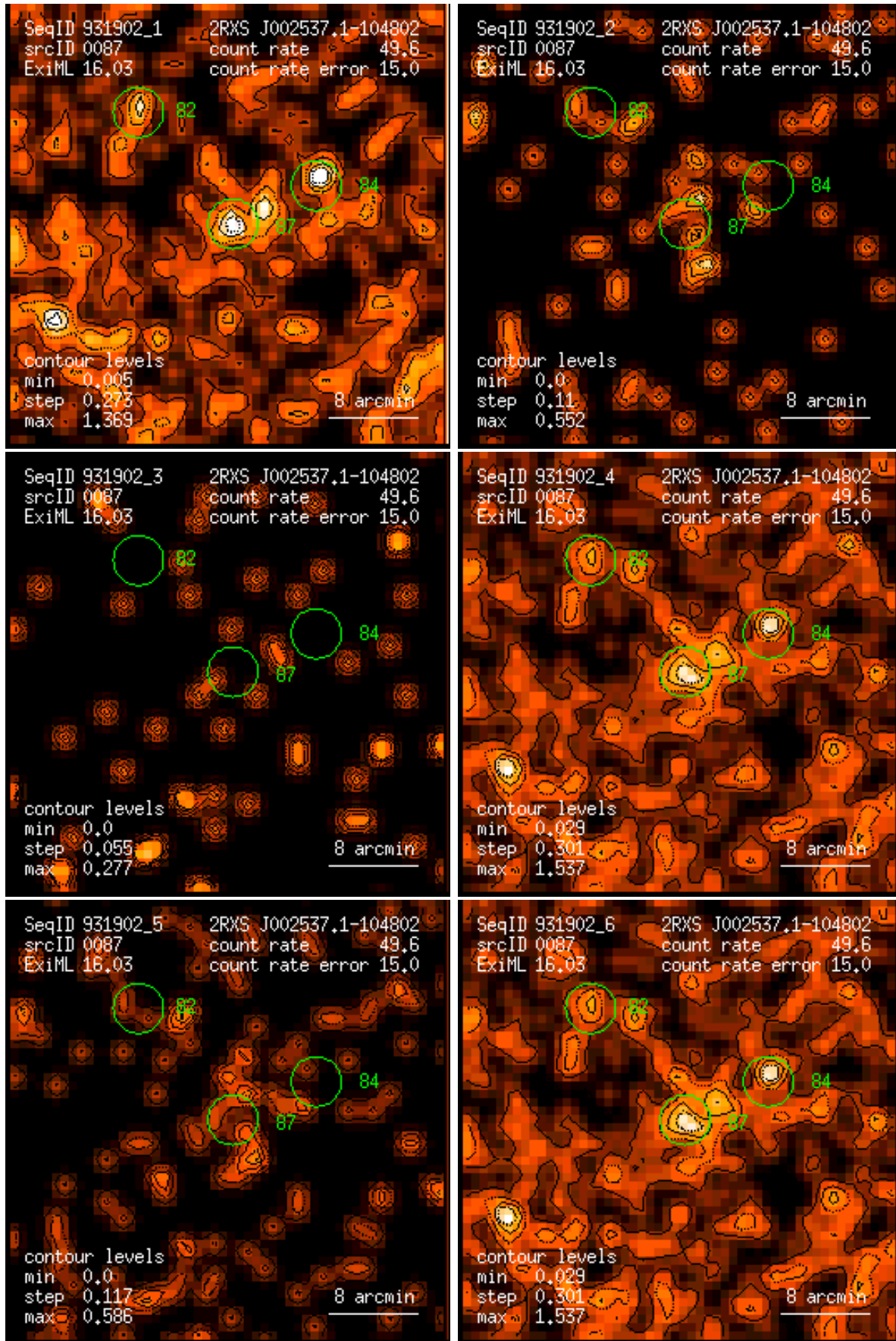
Figure 87: RASS 931902: detection 0087: band rate images, Gaussian filter: (1) PSPC channels 11 – 41, (2) 52 – 90, (3) 91 – 201, (4) 11 – 235, (5) 52 – 201, (6) 11 – 201. Broad band rates in counts/ks. Band rate contour levels in counts/ks/arcmin 2 .
