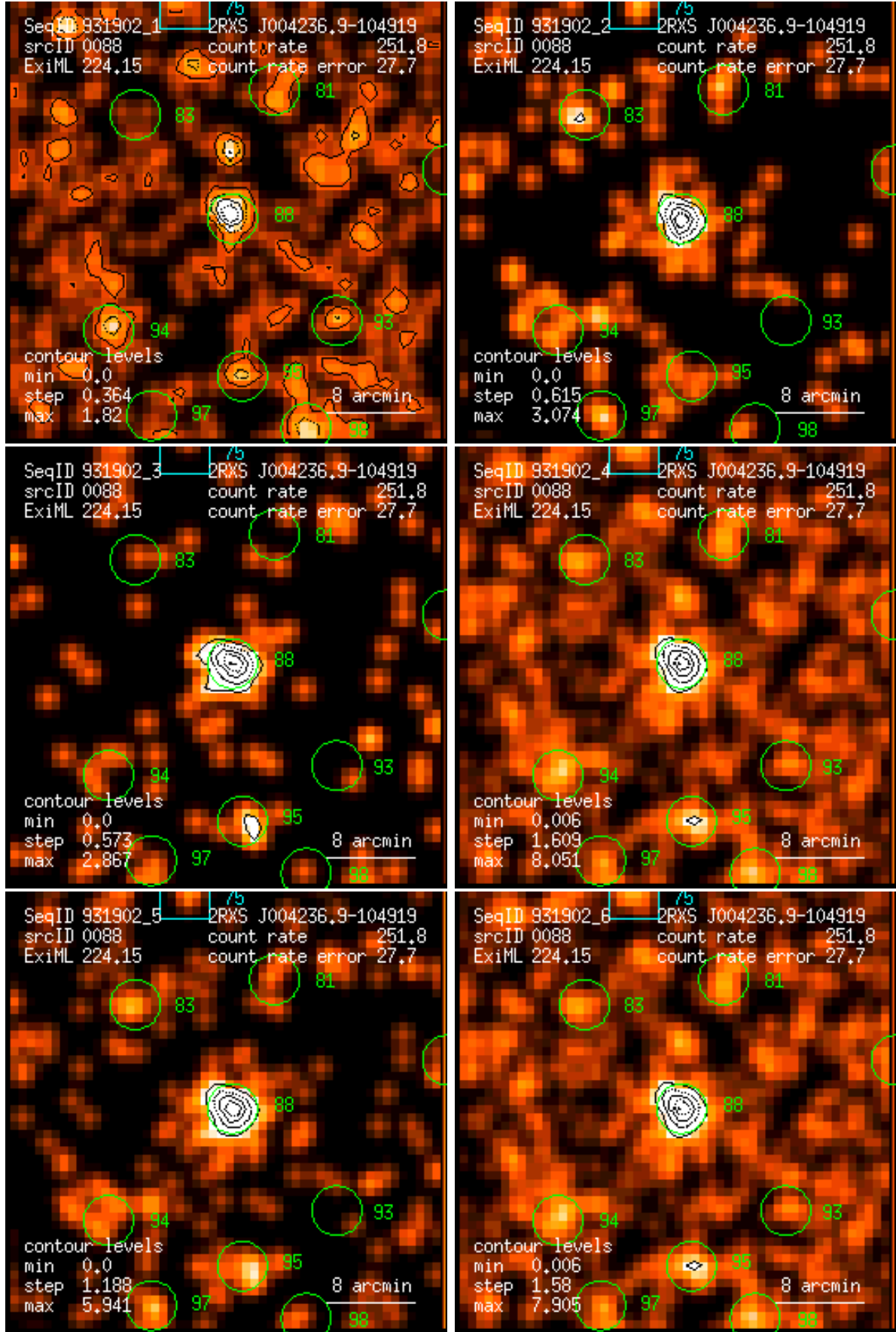
Figure 88: RASS 931902: detection 0088: band rate images, Gaussian filter: (1) PSPC channels 11 – 41, (2) 52 – 90, (3) 91 – 201, (4) 11 – 235, (5) 52 – 201, (6) 11 – 201. Broad band rates in counts/ks. Band rate contour levels in counts/ks/arcmin 2 .
