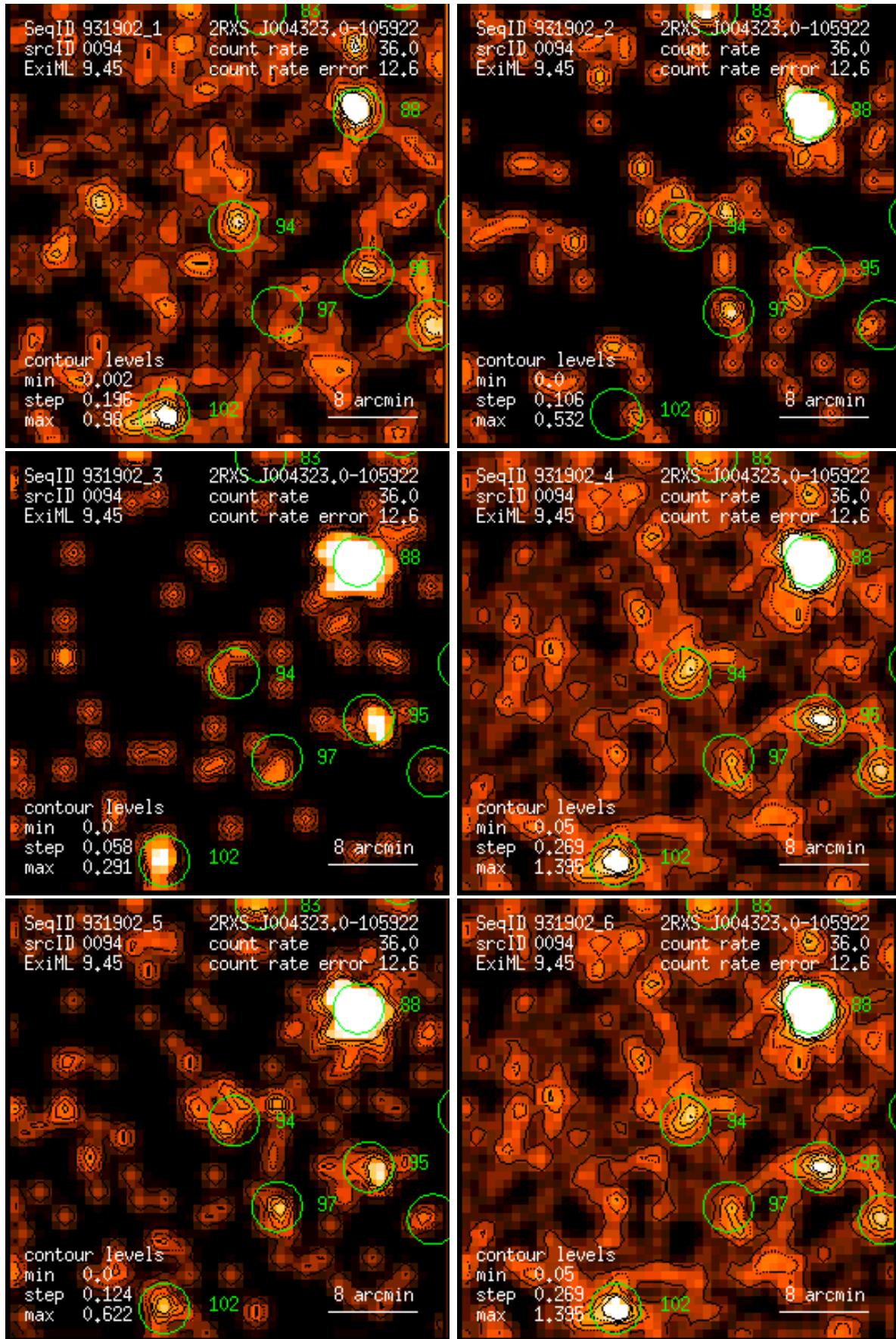
Figure 94: RASS 931902: detection 0094: band rate images, Gaussian filter: (1) PSPC channels 11 – 41, (2) 52 – 90, (3) 91 – 201, (4) 11 – 235, (5) 52 – 201, (6) 11 – 201. Broad band rates in counts/ks. Band rate contour levels in counts/ks/arcmin 2 .
