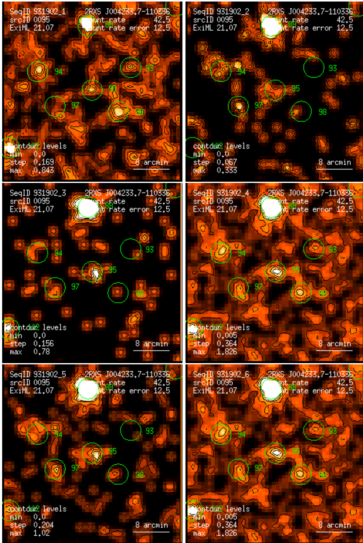
Figure 95: RASS 931902: detection 0095: band rate images, Gaussian filter: (1) PSPC channels 11 – 41, (2) 52 – 90, (3) 91 – 201, (4) 11 – 235, (5) 52 – 201, (6) 11 – 201. Broad band rates in counts/ks. Band rate contour levels in counts/ks/arcmin 2 .
