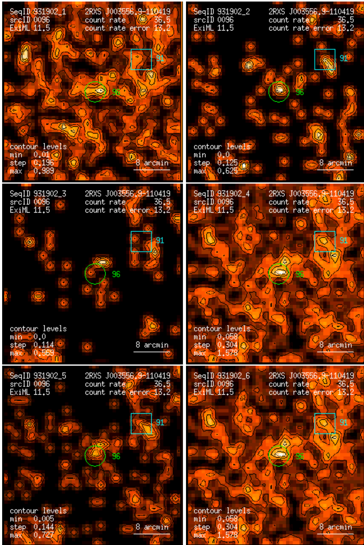
Figure 96: RASS 931902: detection 0096: band rate images, Gaussian filter: (1) PSPC channels 11 – 41, (2) 52 – 90, (3) 91 – 201, (4) 11 – 235, (5) 52 – 201, (6) 11 – 201. Broad band rates in counts/ks. Band rate contour levels in counts/ks/arcmin 2 .
