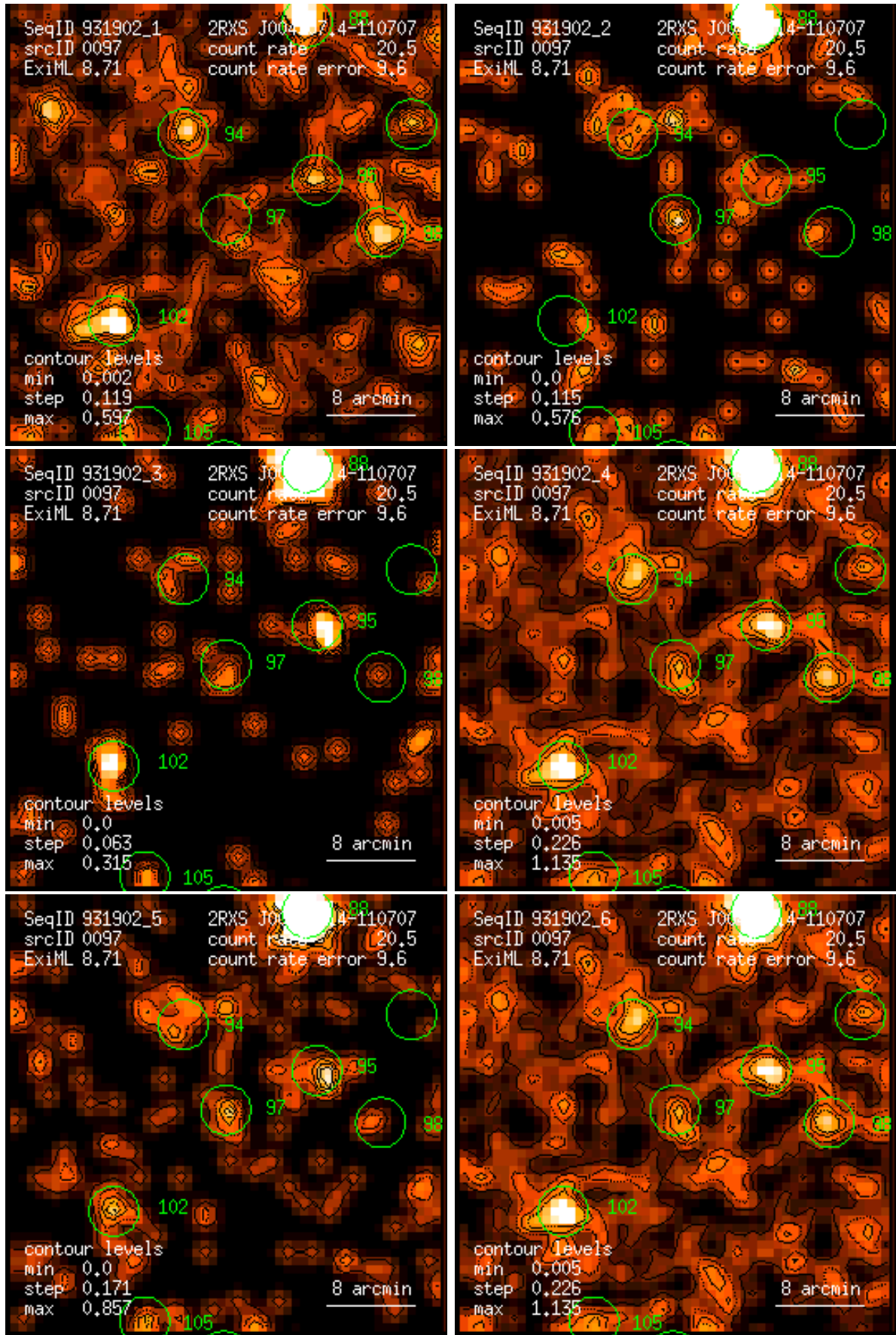
Figure 97: RASS 931902: detection 0097: band rate images, Gaussian filter: (1) PSPC channels 11 – 41, (2) 52 – 90, (3) 91 – 201, (4) 11 – 235, (5) 52 – 201, (6) 11 – 201. Broad band rates in counts/ks. Band rate contour levels in counts/ks/arcmin 2 .
