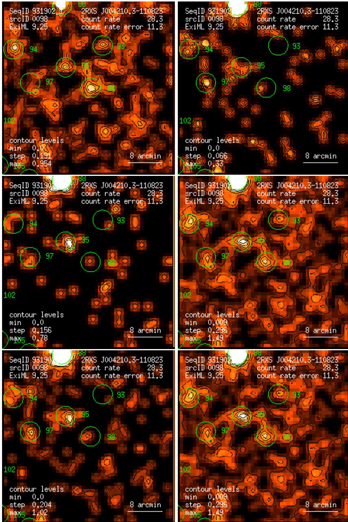
Figure 98: RASS 931902: detection 0098: band rate images, Gaussian filter: (1) PSPC channels 11 – 41, (2) 52 – 90, (3) 91 – 201, (4) 11 – 235, (5) 52 – 201, (6) 11 – 201. Broad band rates in counts/ks. Band rate contour levels in counts/ks/arcmin 2 .
