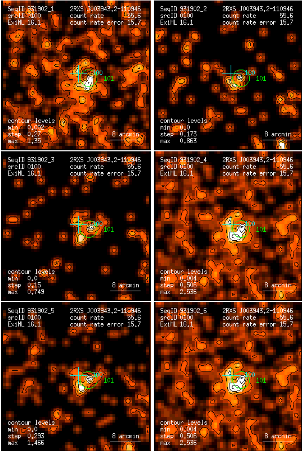
Figure 100: RASS 931902: detection 0100: band rate images, Gaussian filter: (1) PSPC channels 11 – 41, (2) 52 – 90, (3) 91 – 201, (4) 11 – 235, (5) 52 – 201, (6) 11 – 201. Broad band rates in counts/ks. Band rate contour levels in counts/ks/arcmin 2 .
