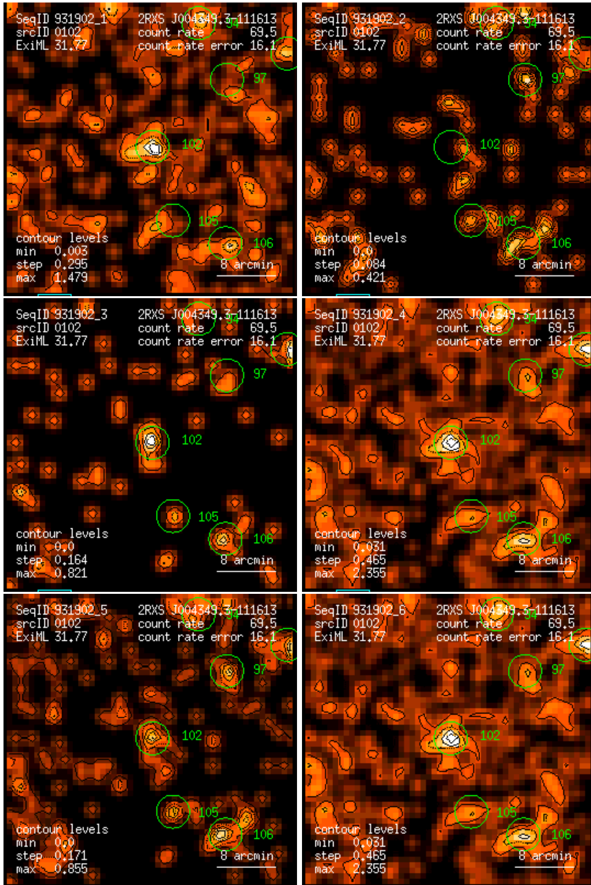
Figure 102: RASS 931902: detection 0102: band rate images, Gaussian filter: (1) PSPC channels 11 – 41, (2) 52 – 90, (3) 91 – 201, (4) 11 – 235, (5) 52 – 201, (6) 11 – 201. Broad band rates in counts/ks. Band rate contour levels in counts/ks/arcmin 2 .
