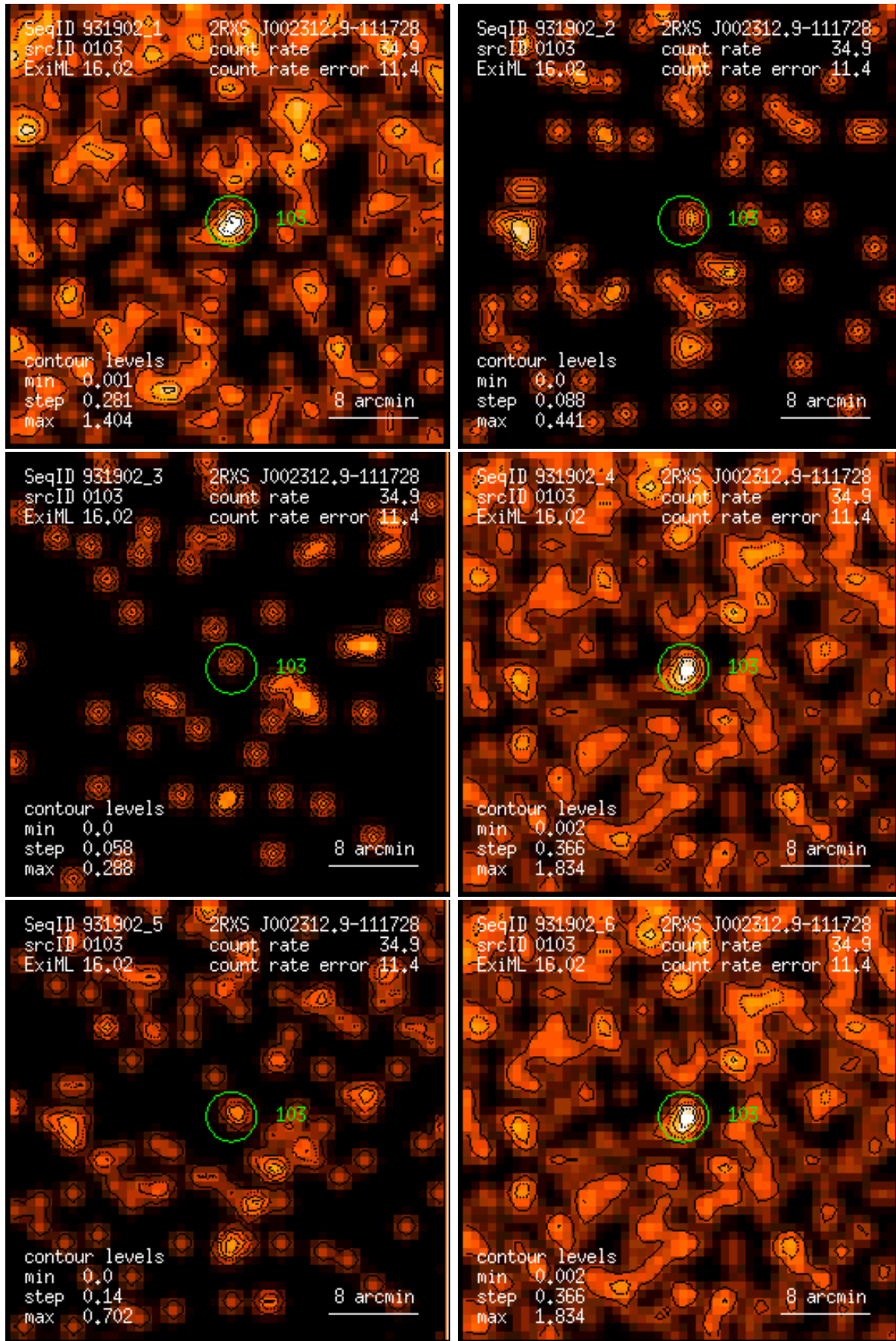
Figure 103: RASS 931902: detection 0103: band rate images, Gaussian filter: (1) PSPC channels 11 – 41, (2) 52 – 90, (3) 91 – 201, (4) 11 – 235, (5) 52 – 201, (6) 11 – 201. Broad band rates in counts/ks. Band rate contour levels in counts/ks/arcmin 2 .
