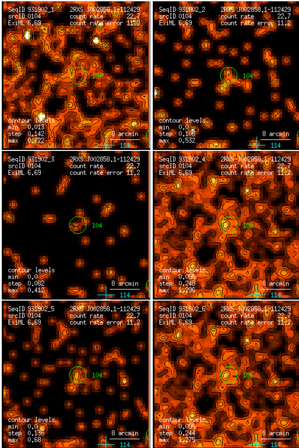
Figure 104: RASS 931902: detection 0104: band rate images, Gaussian filter: (1) PSPC channels 11 – 41, (2) 52 – 90, (3) 91 – 201, (4) 11 – 235, (5) 52 – 201, (6) 11 – 201. Broad band rates in counts/ks. Band rate contour levels in counts/ks/arcmin 2 .
