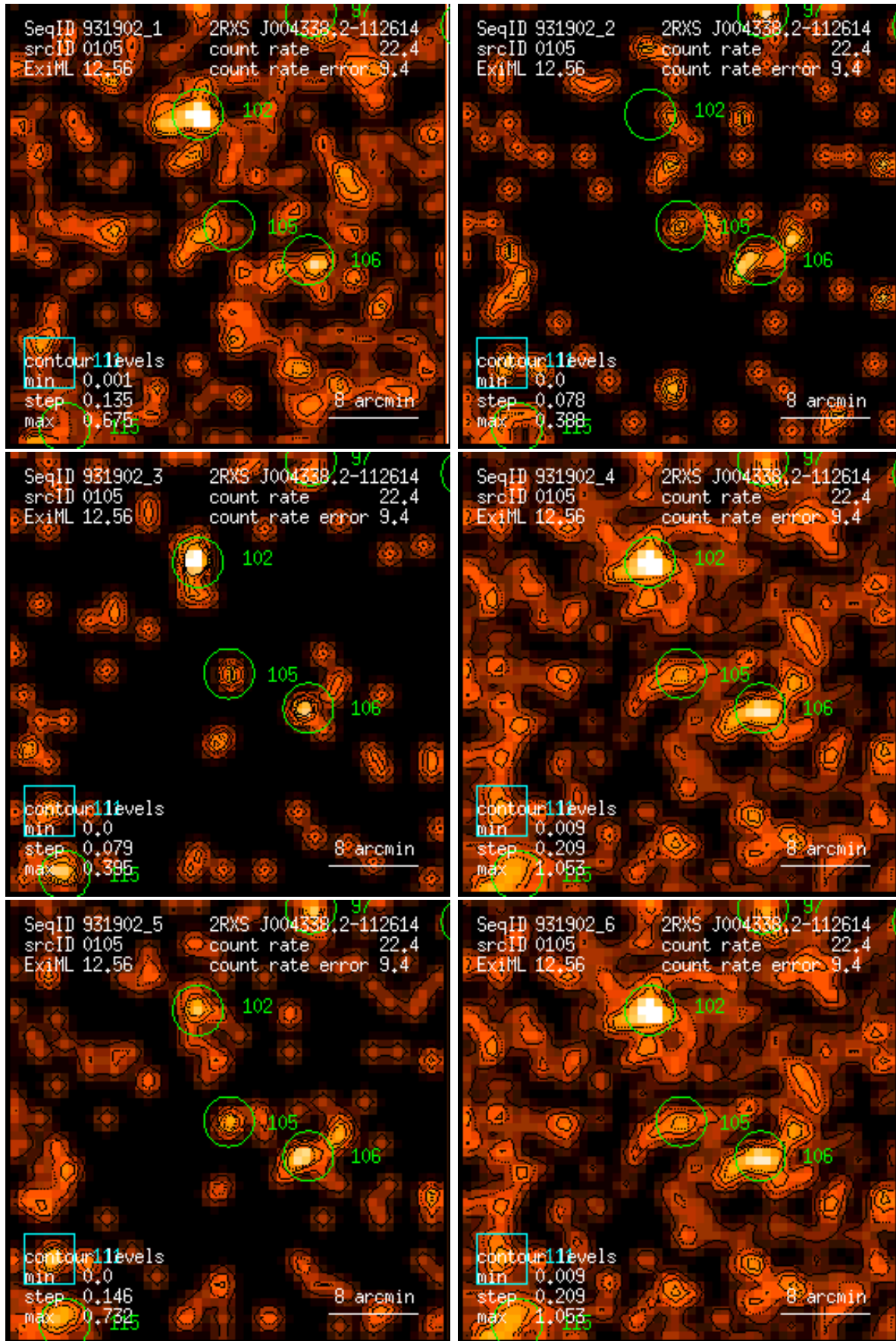
Figure 105: RASS 931902: detection 0105: band rate images, Gaussian filter: (1) PSPC channels 11 – 41, (2) 52 – 90, (3) 91 – 201, (4) 11 – 235, (5) 52 – 201, (6) 11 – 201. Broad band rates in counts/ks. Band rate contour levels in counts/ks/arcmin 2 .
