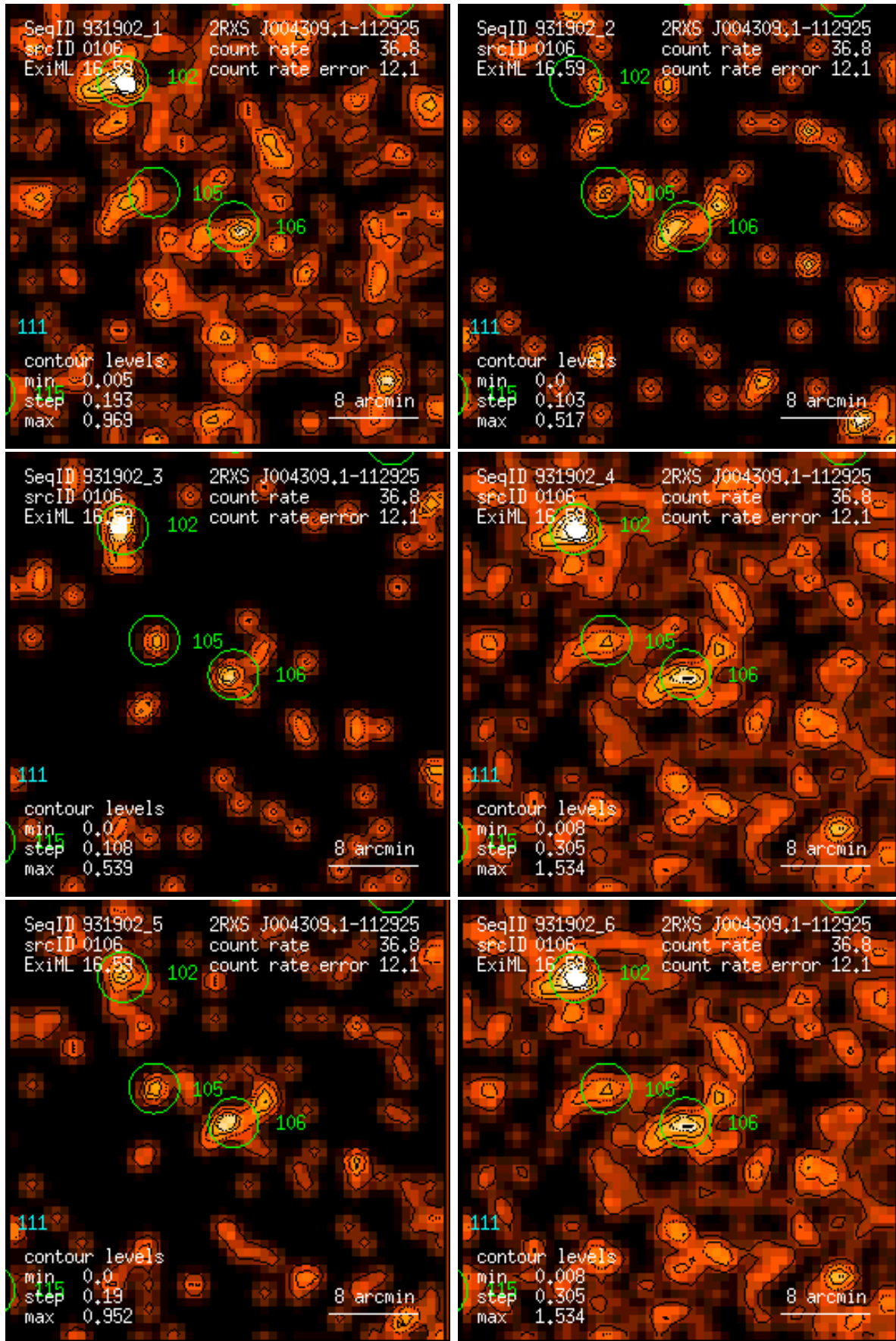
Figure 106: RASS 931902: detection 0106: band rate images, Gaussian filter: (1) PSPC channels 11 – 41, (2) 52 – 90, (3) 91 – 201, (4) 11 – 235, (5) 52 – 201, (6) 11 – 201. Broad band rates in counts/ks. Band rate contour levels in counts/ks/arcmin 2 .
