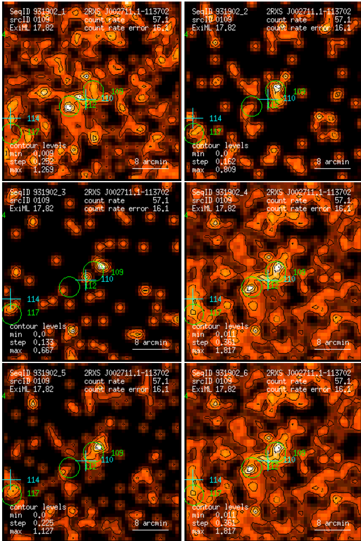
Figure 109: RASS 931902: detection 0109: band rate images, Gaussian filter: (1) PSPC channels 11 – 41, (2) 52 – 90, (3) 91 – 201, (4) 11 – 235, (5) 52 – 201, (6) 11 – 201. Broad band rates in counts/ks. Band rate contour levels in counts/ks/arcmin 2 .
