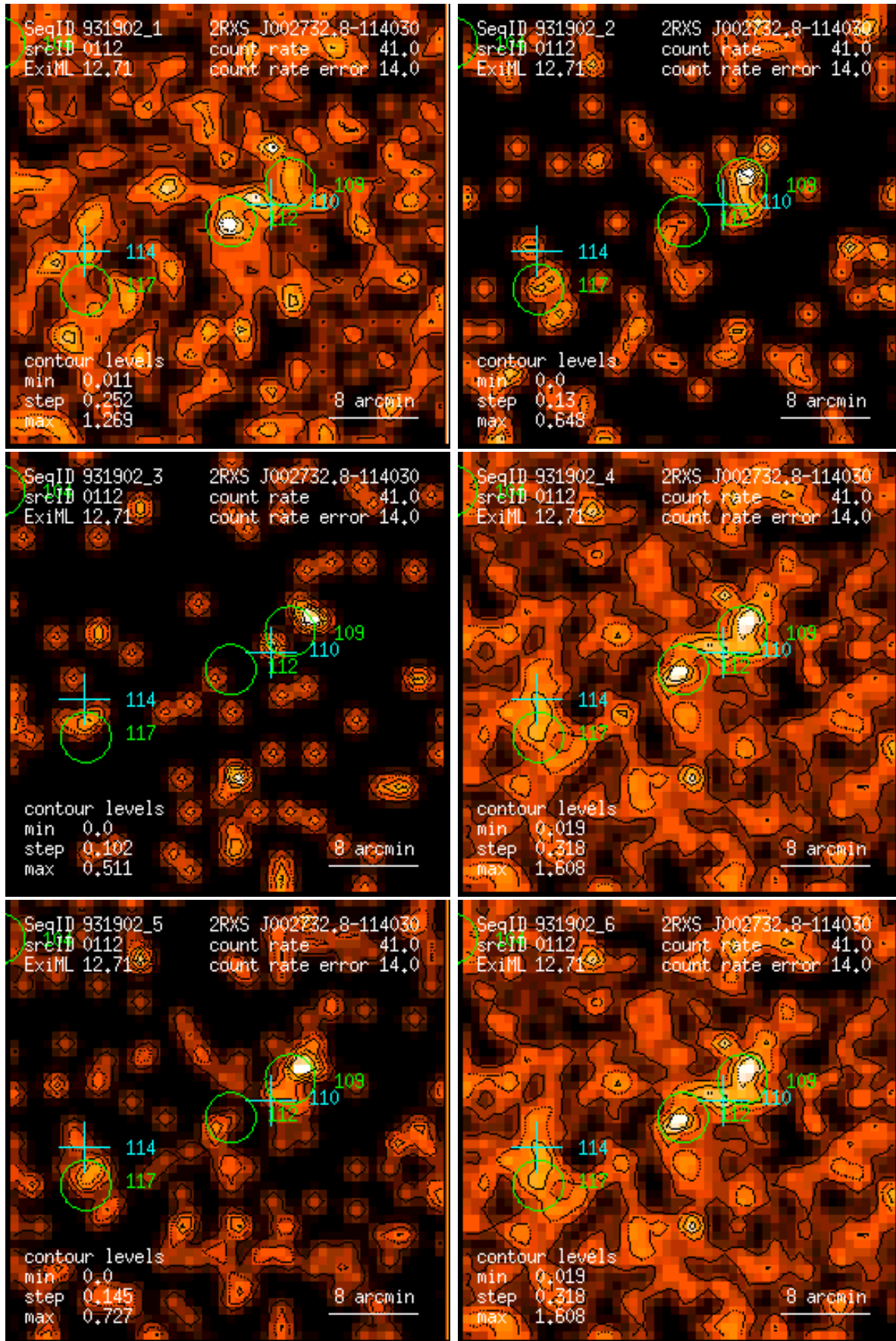
Figure 112: RASS 931902: detection 0112: band rate images, Gaussian filter: (1) PSPC channels 11 – 41, (2) 52 – 90, (3) 91 – 201, (4) 11 – 235, (5) 52 – 201, (6) 11 – 201. Broad band rates in counts/ks. Band rate contour levels in counts/ks/arcmin 2 .
