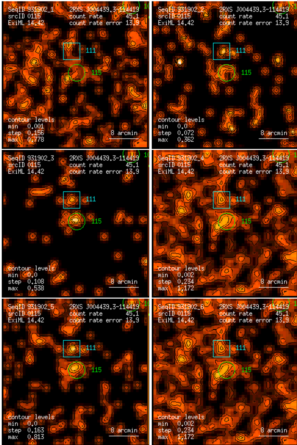
Figure 115: RASS 931902: detection 0115: band rate images, Gaussian filter: (1) PSPC channels 11 – 41, (2) 52 – 90, (3) 91 – 201, (4) 11 – 235, (5) 52 – 201, (6) 11 – 201. Broad band rates in counts/ks. Band rate contour levels in counts/ks/arcmin 2 .
