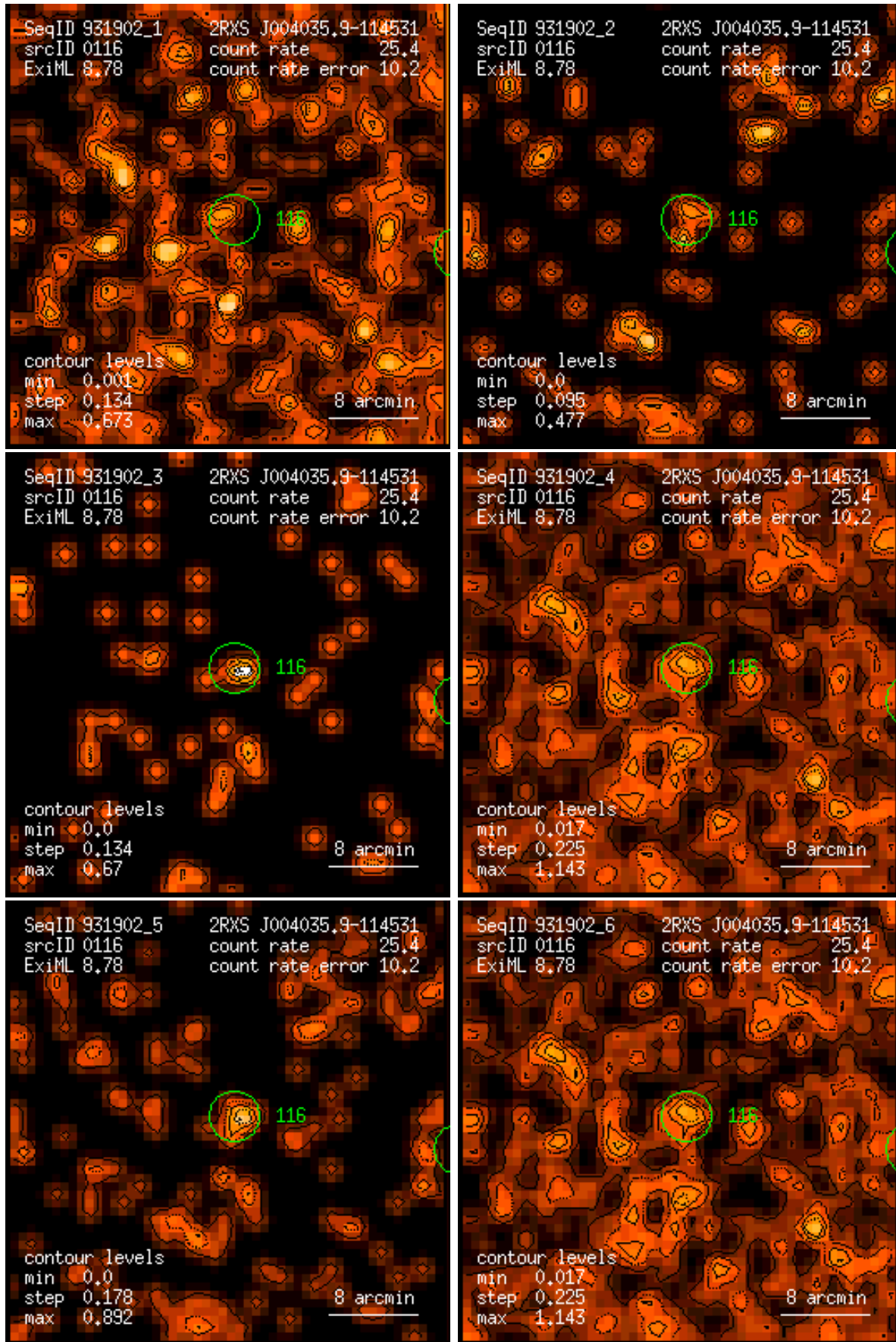
Figure 116: RASS 931902: detection 0116: band rate images, Gaussian filter: (1) PSPC channels 11 – 41, (2) 52 – 90, (3) 91 – 201, (4) 11 – 235, (5) 52 – 201, (6) 11 – 201. Broad band rates in counts/ks. Band rate contour levels in counts/ks/arcmin 2 .
