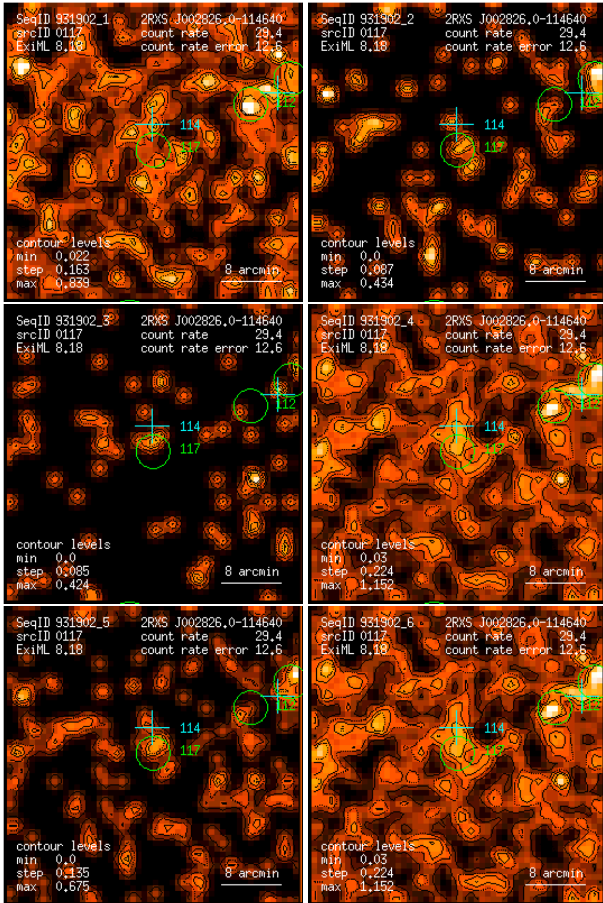
Figure 117: RASS 931902: detection 0117: band rate images, Gaussian filter: (1) PSPC channels 11 – 41, (2) 52 – 90, (3) 91 – 201, (4) 11 – 235, (5) 52 – 201, (6) 11 – 201. Broad band rates in counts/ks. Band rate contour levels in counts/ks/arcmin 2 .
