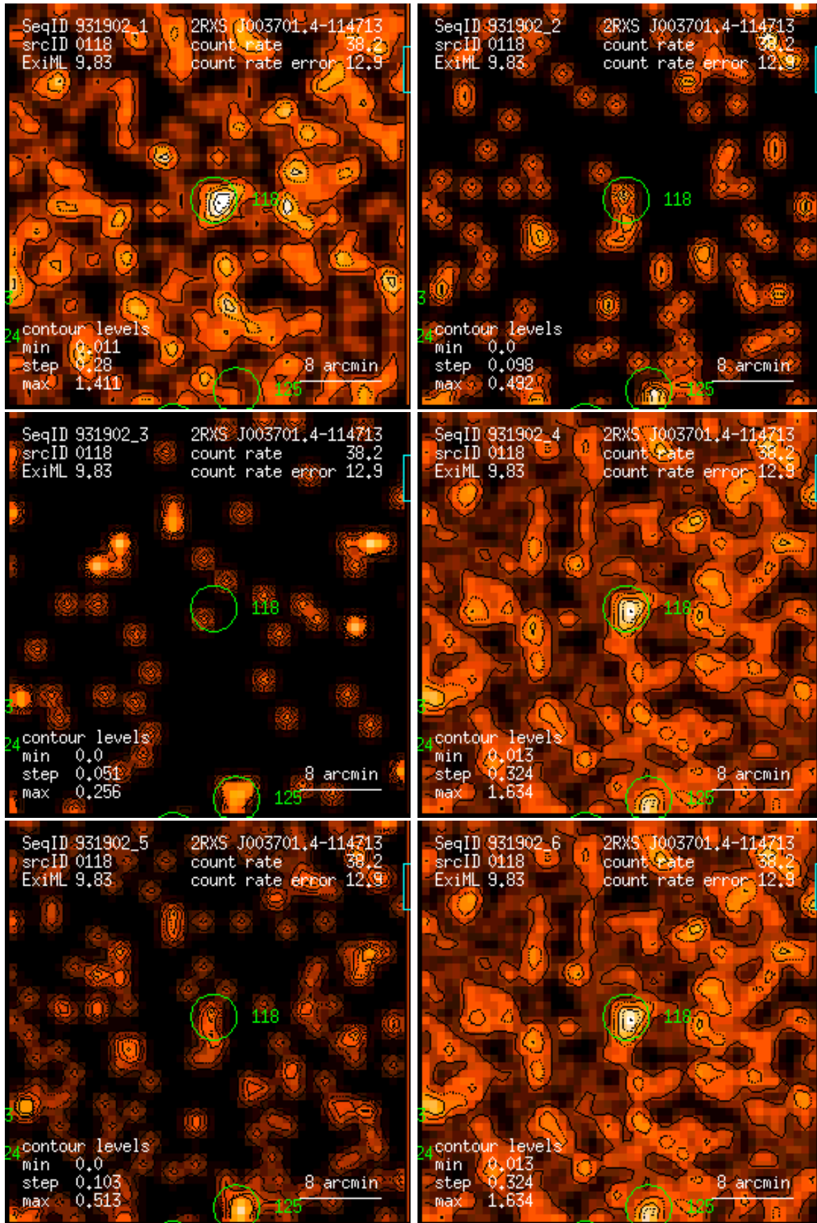
Figure 118: RASS 931902: detection 0118: band rate images, Gaussian filter: (1) PSPC channels 11 – 41, (2) 52 – 90, (3) 91 – 201, (4) 11 – 235, (5) 52 – 201, (6) 11 – 201. Broad band rates in counts/ks. Band rate contour levels in counts/ks/arcmin 2 .
