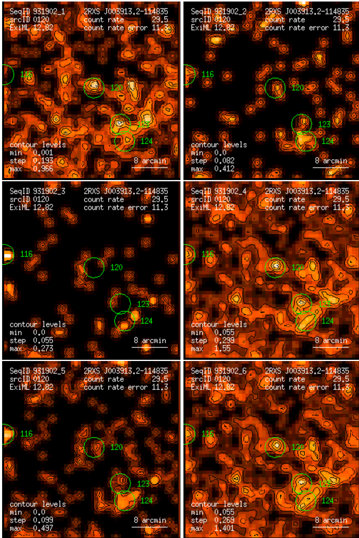
Figure 120: RASS 931902: detection 0120: band rate images, Gaussian filter: (1) PSPC channels 11 – 41, (2) 52 – 90, (3) 91 – 201, (4) 11 – 235, (5) 52 – 201, (6) 11 – 201. Broad band rates in counts/ks. Band rate contour levels in counts/ks/arcmin 2 .
