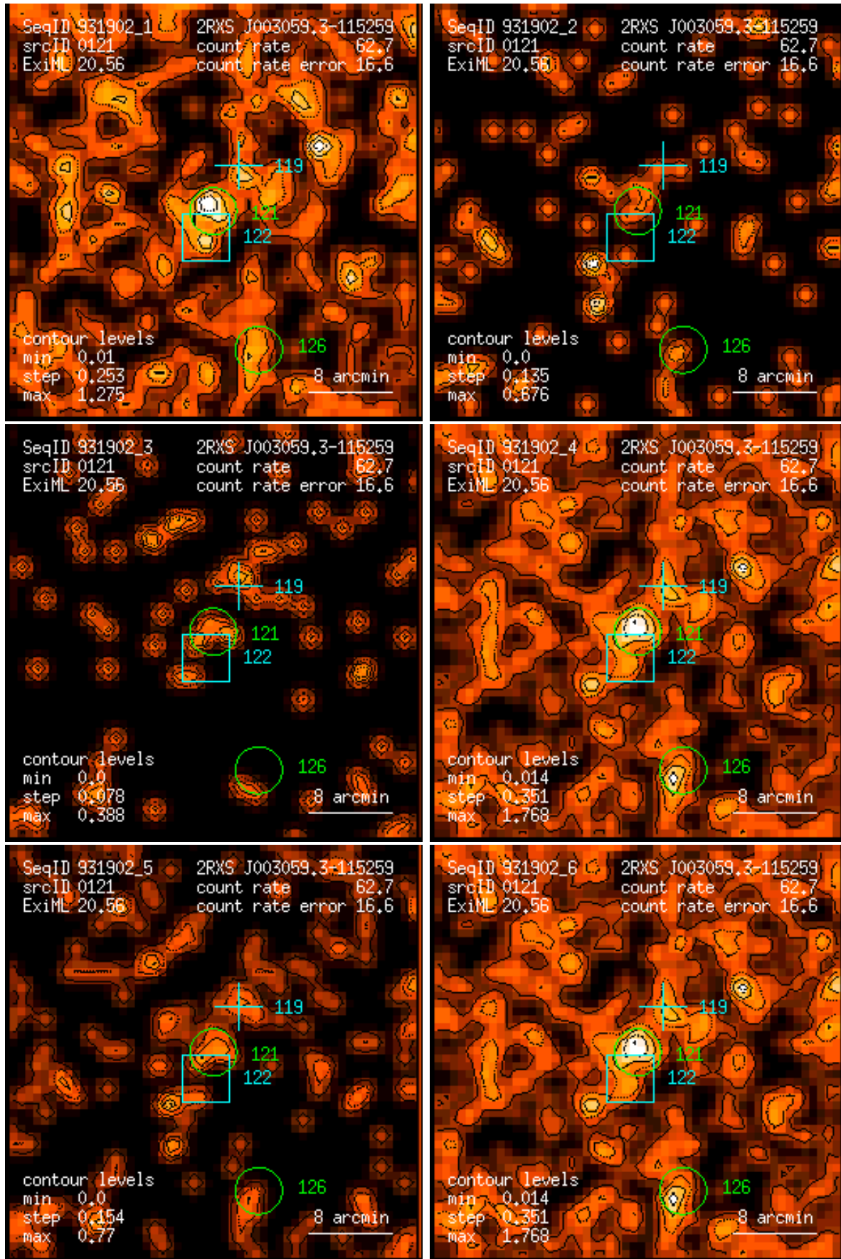
Figure 121: RASS 931902: detection 0121: band rate images, Gaussian filter: (1) PSPC channels 11 – 41, (2) 52 – 90, (3) 91 – 201, (4) 11 – 235, (5) 52 – 201, (6) 11 – 201. Broad band rates in counts/ks. Band rate contour levels in counts/ks/arcmin 2 .
