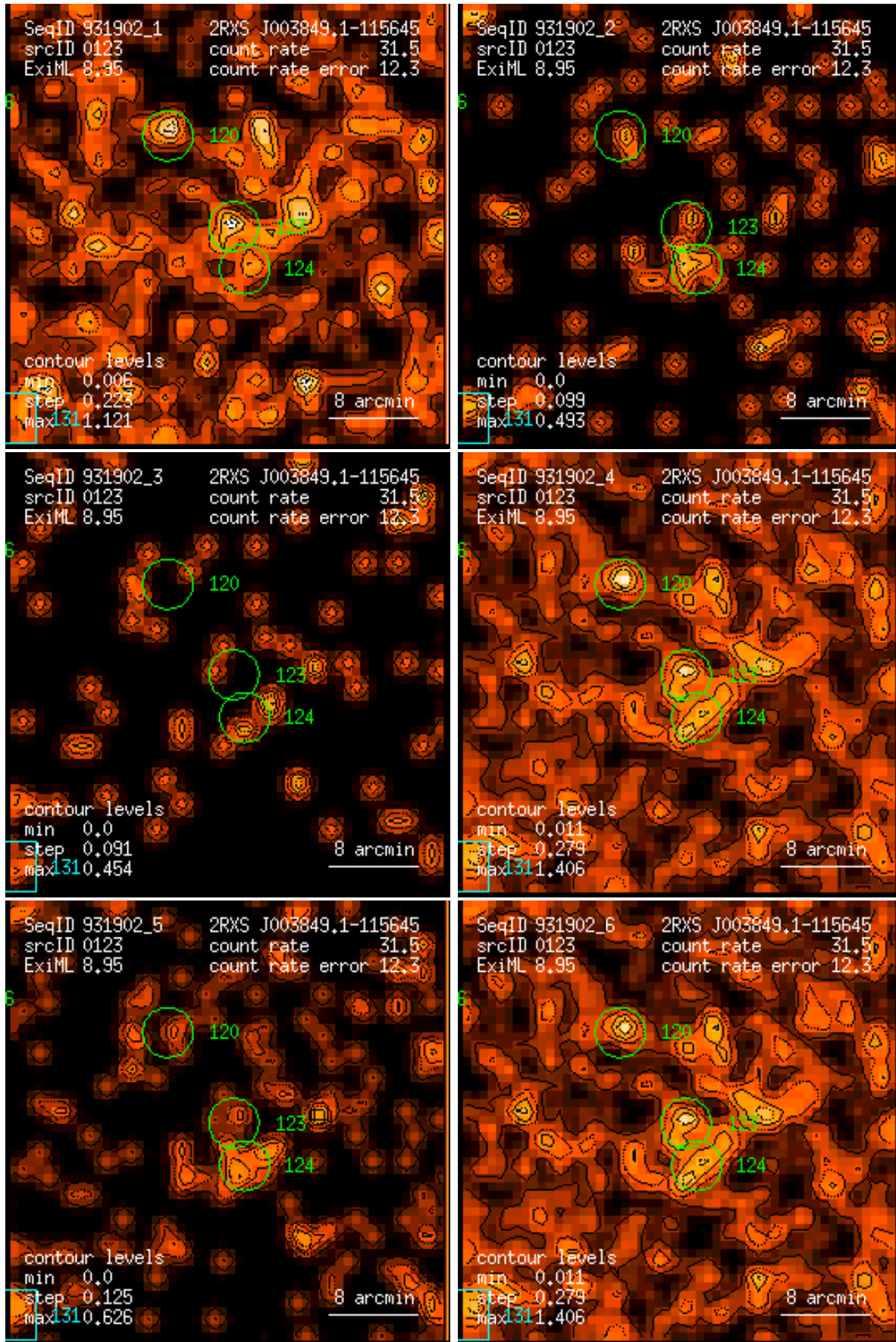
Figure 123: RASS 931902: detection 0123: band rate images, Gaussian filter: (1) PSPC channels 11 – 41, (2) 52 – 90, (3) 91 – 201, (4) 11 – 235, (5) 52 – 201, (6) 11 – 201. Broad band rates in counts/ks. Band rate contour levels in counts/ks/arcmin 2 .
