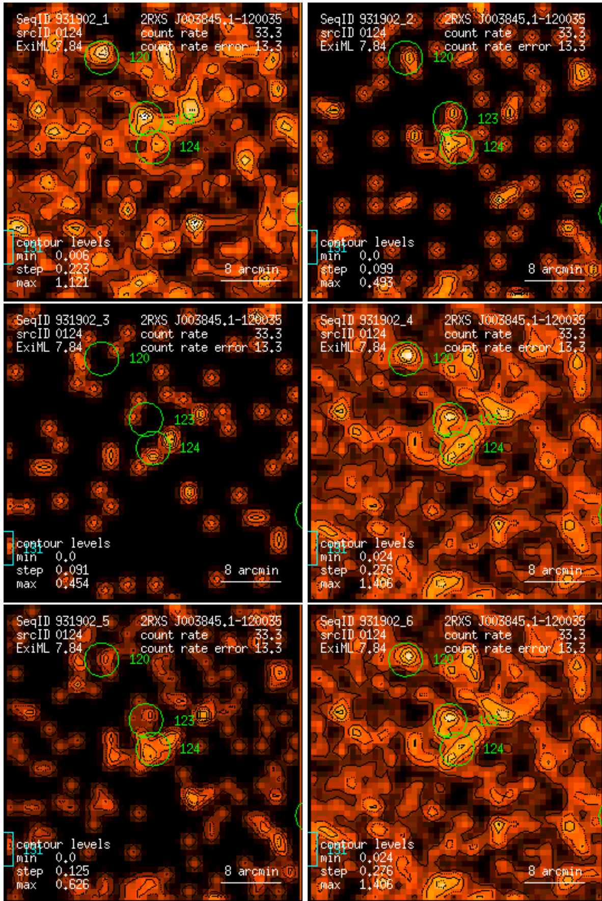
Figure 124: RASS 931902: detection 0124: band rate images, Gaussian filter: (1) PSPC channels 11 – 41, (2) 52 – 90, (3) 91 – 201, (4) 11 – 235, (5) 52 – 201, (6) 11 – 201. Broad band rates in counts/ks. Band rate contour levels in counts/ks/arcmin 2 .
