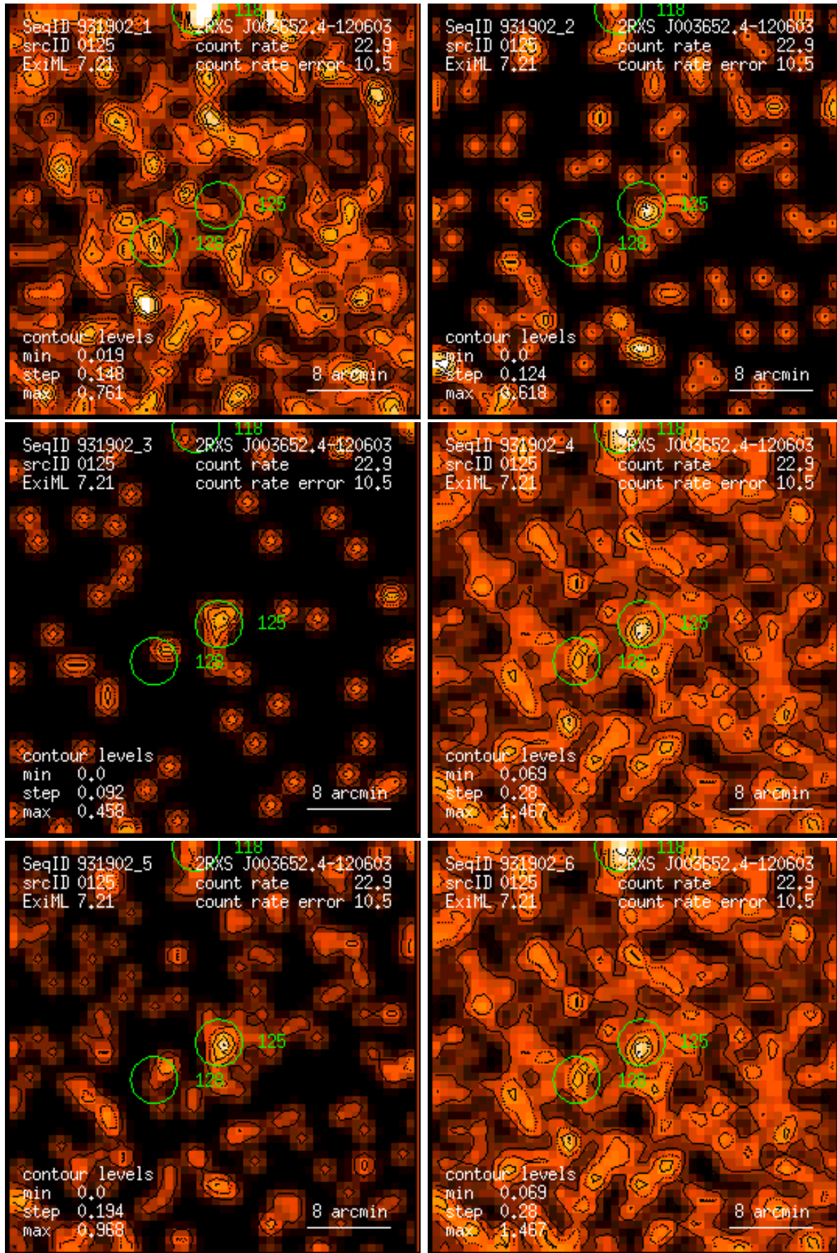
Figure 125: RASS 931902: detection 0125: band rate images, Gaussian filter: (1) PSPC channels 11 – 41, (2) 52 – 90, (3) 91 – 201, (4) 11 – 235, (5) 52 – 201, (6) 11 – 201. Broad band rates in counts/ks. Band rate contour levels in counts/ks/arcmin 2 .
