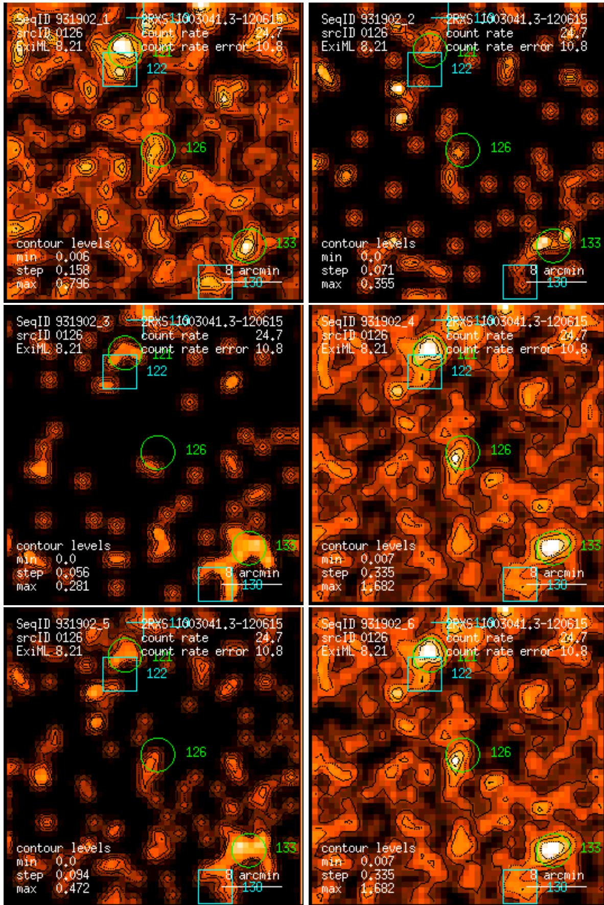
Figure 126: RASS 931902: detection 0126: band rate images, Gaussian filter: (1) PSPC channels 11 – 41, (2) 52 – 90, (3) 91 – 201, (4) 11 – 235, (5) 52 – 201, (6) 11 – 201. Broad band rates in counts/ks. Band rate contour levels in counts/ks/arcmin 2 .
