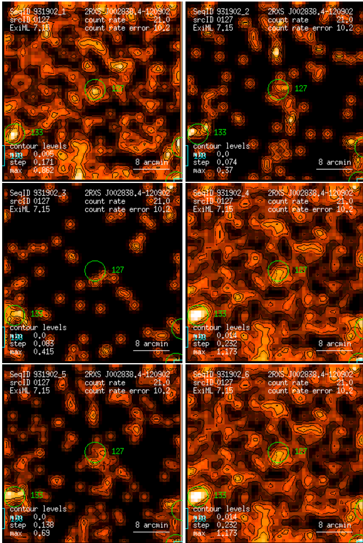
Figure 127: RASS 931902: detection 0127: band rate images, Gaussian filter: (1) PSPC channels 11 – 41, (2) 52 – 90, (3) 91 – 201, (4) 11 – 235, (5) 52 – 201, (6) 11 – 201. Broad band rates in counts/ks. Band rate contour levels in counts/ks/arcmin 2 .
