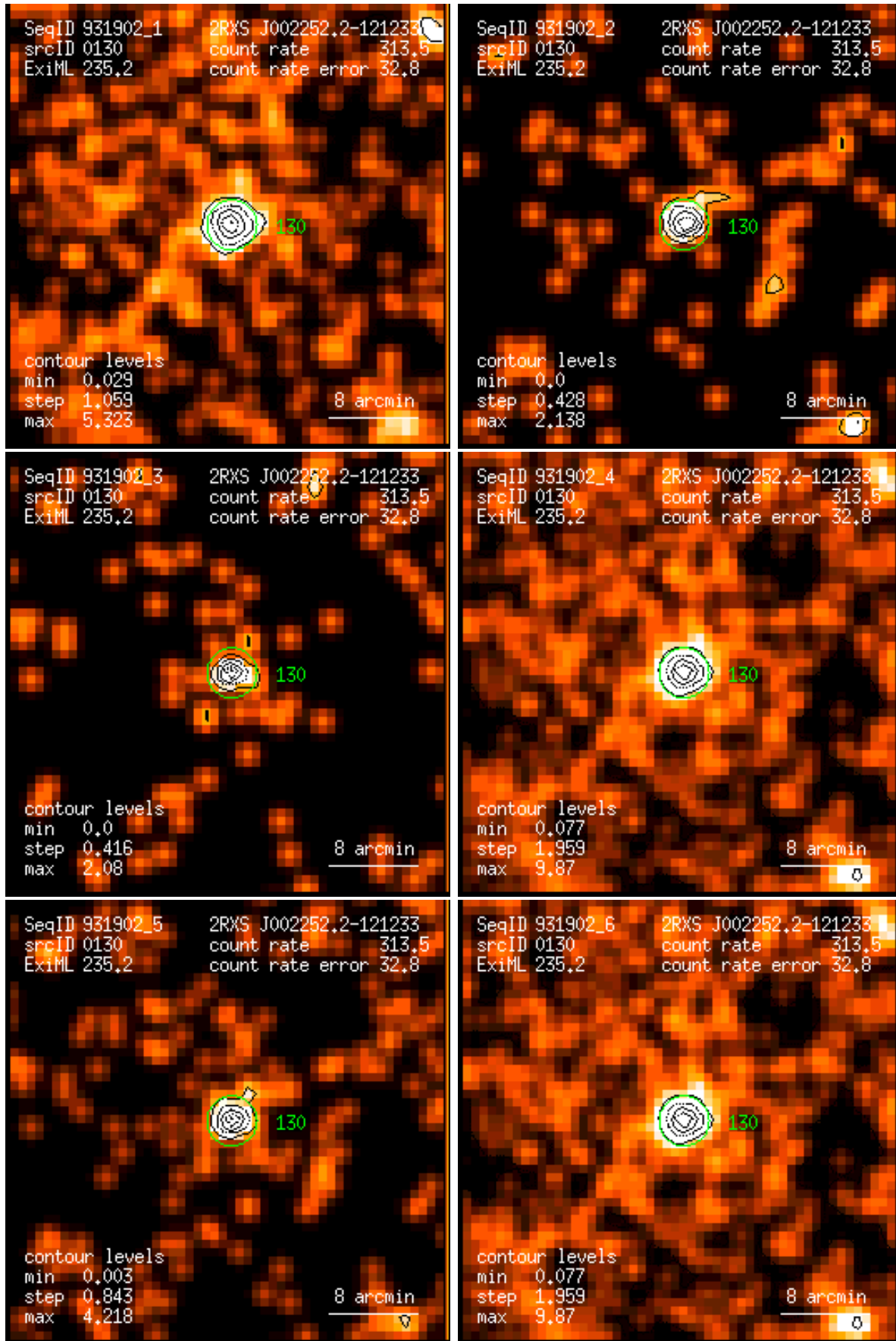
Figure 130: RASS 931902: detection 0130: band rate images, Gaussian filter: (1) PSPC channels 11 – 41, (2) 52 – 90, (3) 91 – 201, (4) 11 – 235, (5) 52 – 201, (6) 11 – 201. Broad band rates in counts/ks. Band rate contour levels in counts/ks/arcmin 2 .
