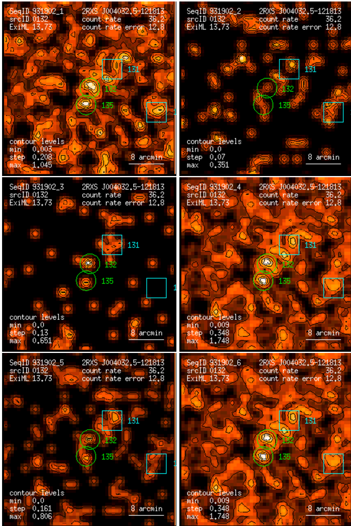
Figure 132: RASS 931902: detection 0132: band rate images, Gaussian filter: (1) PSPC channels 11 – 41, (2) 52 – 90, (3) 91 – 201, (4) 11 – 235, (5) 52 – 201, (6) 11 – 201. Broad band rates in counts/ks. Band rate contour levels in counts/ks/arcmin 2 .
