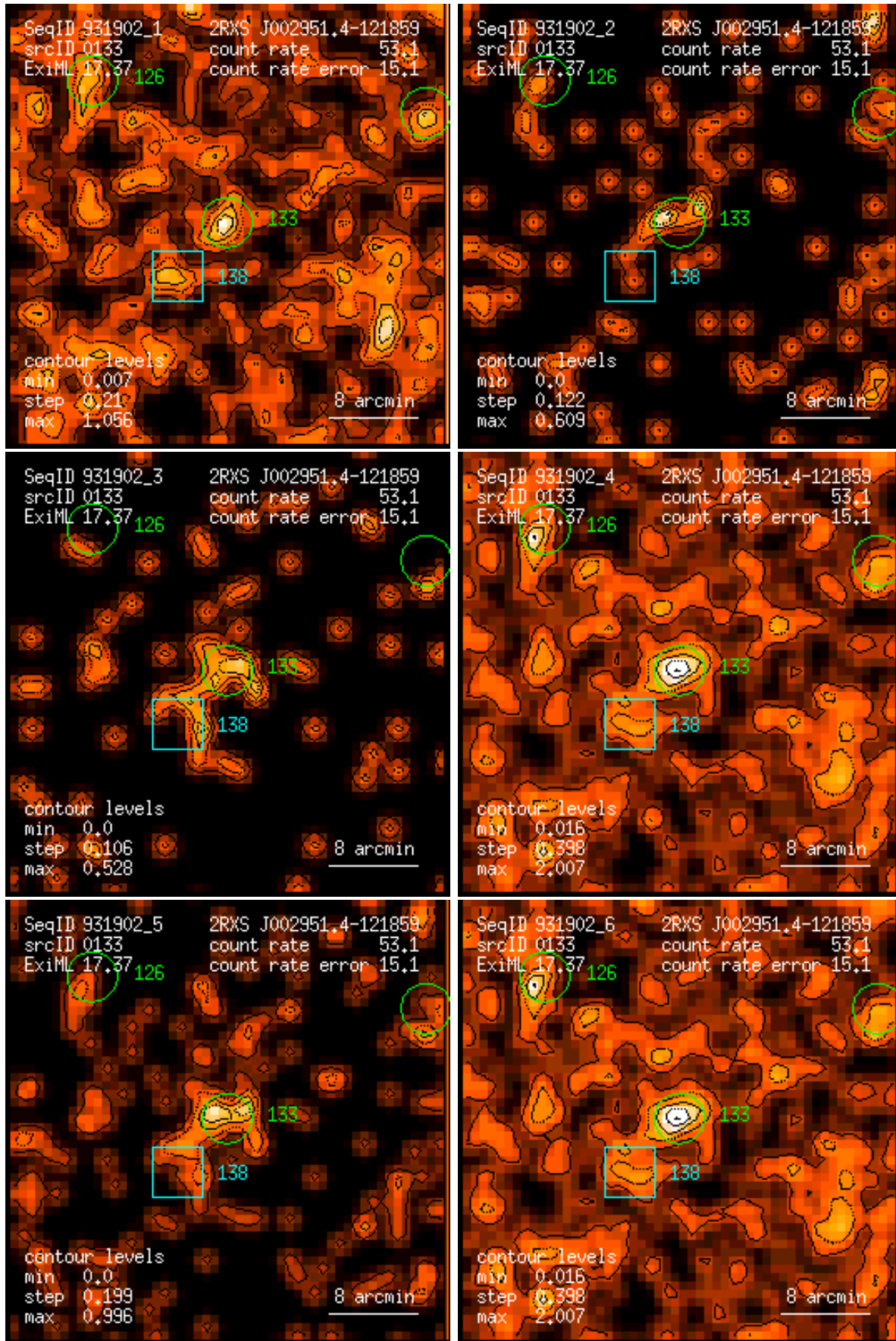
Figure 133: RASS 931902: detection 0133: band rate images, Gaussian filter: (1) PSPC channels 11 – 41, (2) 52 – 90, (3) 91 – 201, (4) 11 – 235, (5) 52 – 201, (6) 11 – 201. Broad band rates in counts/ks. Band rate contour levels in counts/ks/arcmin 2 .
