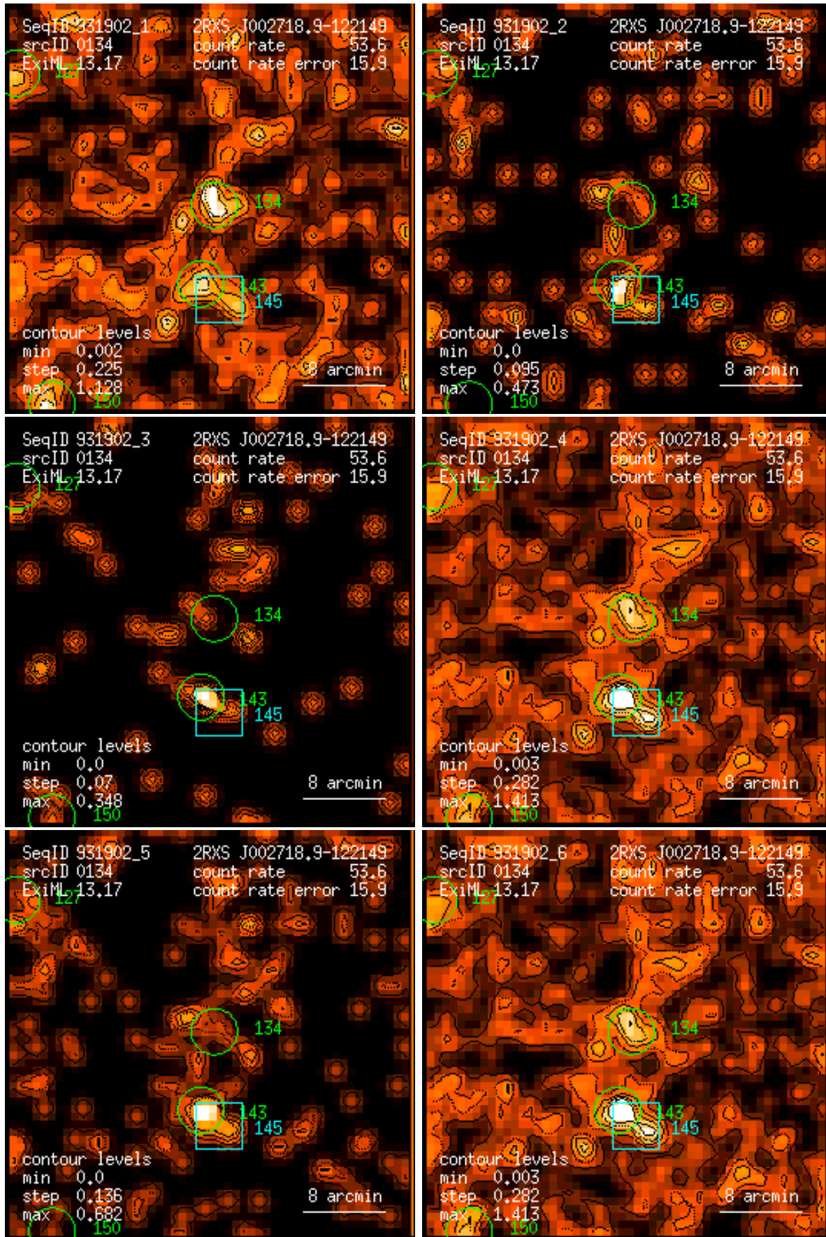
Figure 134: RASS 931902: detection 0134: band rate images, Gaussian filter: (1) PSPC channels 11 – 41, (2) 52 – 90, (3) 91 – 201, (4) 11 – 235, (5) 52 – 201, (6) 11 – 201. Broad band rates in counts/ks. Band rate contour levels in counts/ks/arcmin 2 .
