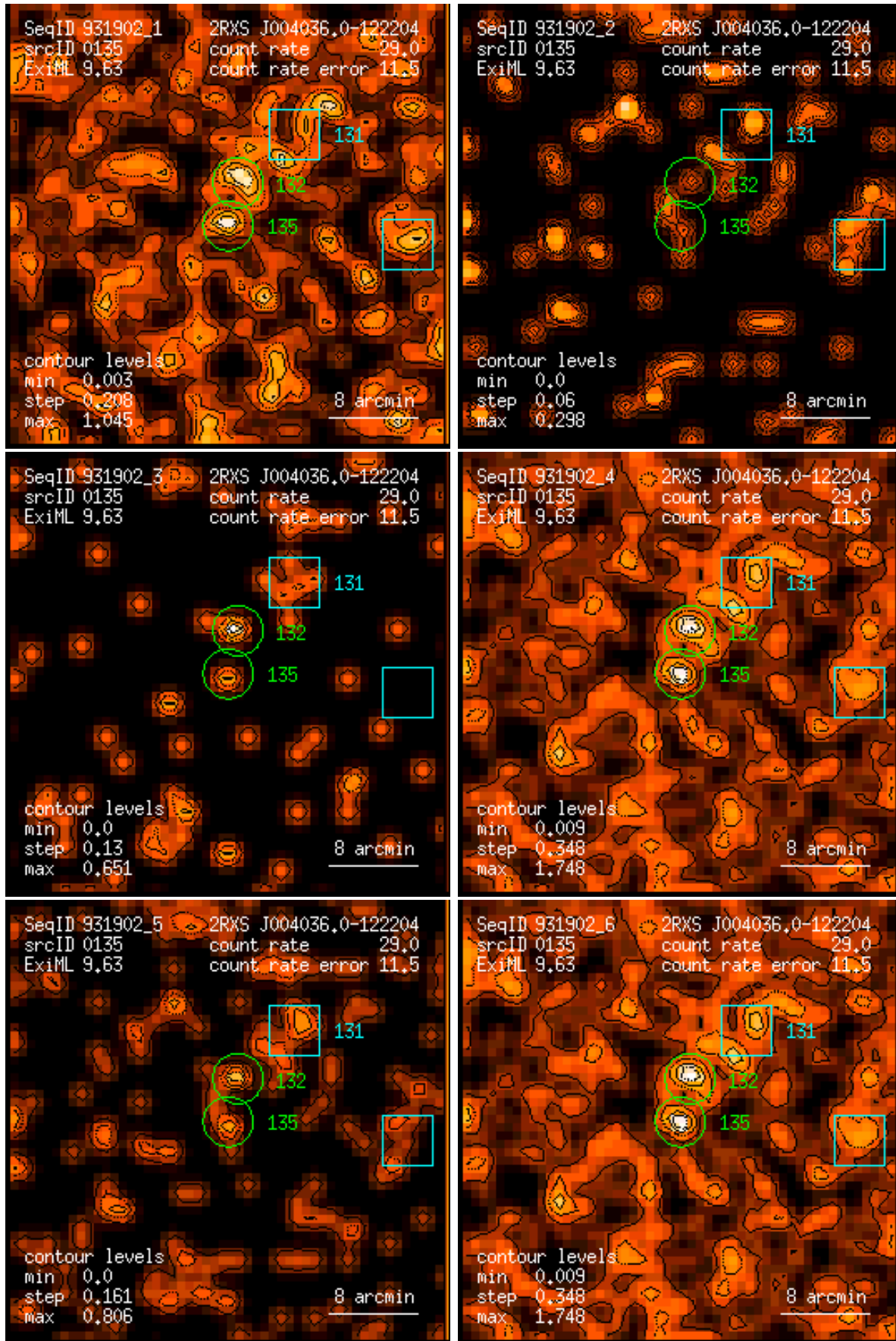
Figure 135: RASS 931902: detection 0135: band rate images, Gaussian filter: (1) PSPC channels 11 – 41, (2) 52 – 90, (3) 91 – 201, (4) 11 – 235, (5) 52 – 201, (6) 11 – 201. Broad band rates in counts/ks. Band rate contour levels in counts/ks/arcmin 2 .
