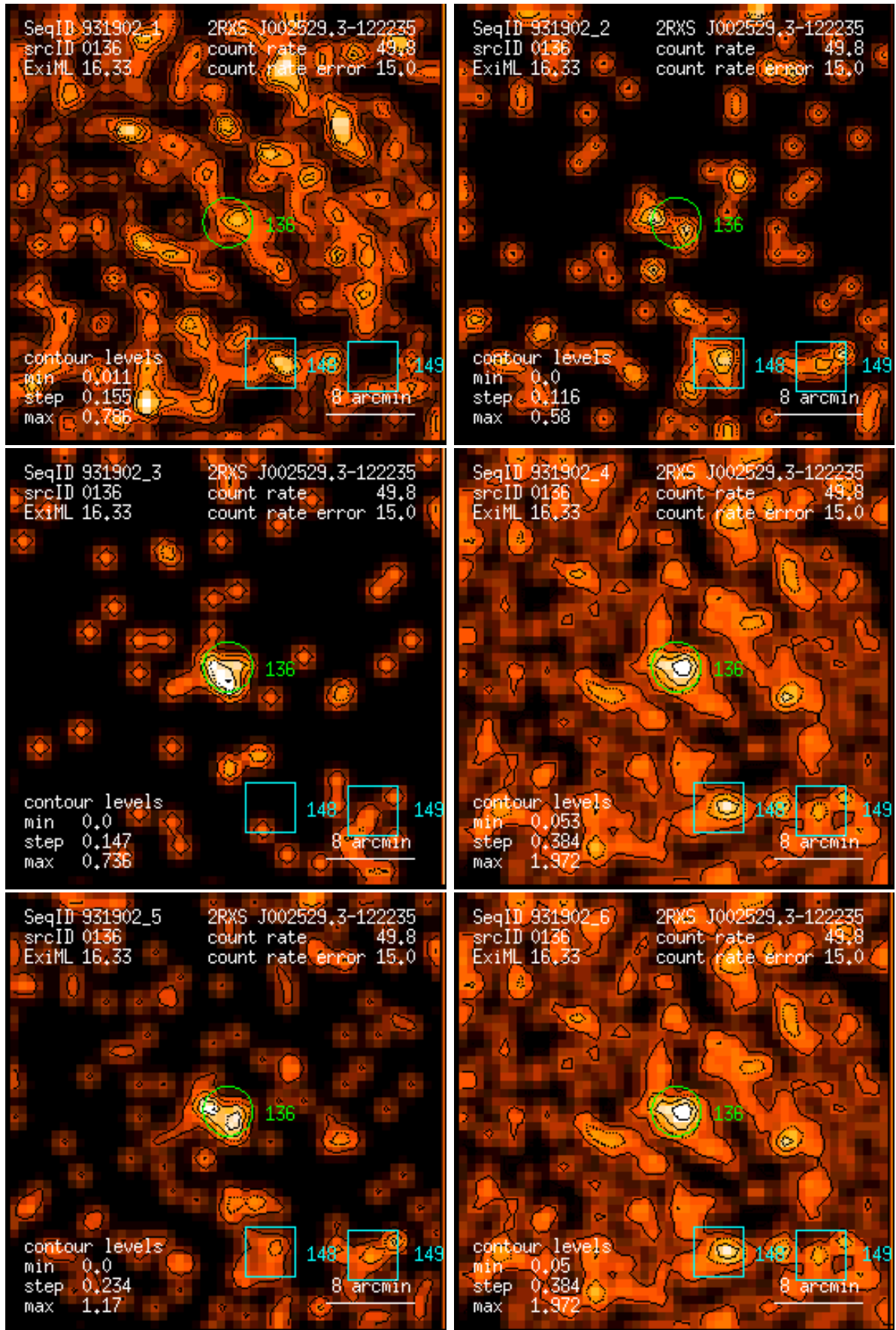
Figure 136: RASS 931902: detection 0136: band rate images, Gaussian filter: (1) PSPC channels 11 – 41, (2) 52 – 90, (3) 91 – 201, (4) 11 – 235, (5) 52 – 201, (6) 11 – 201. Broad band rates in counts/ks. Band rate contour levels in counts/ks/arcmin 2 .
